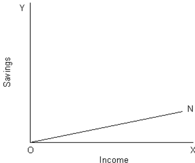
Fig 3.2 saving-income curve
