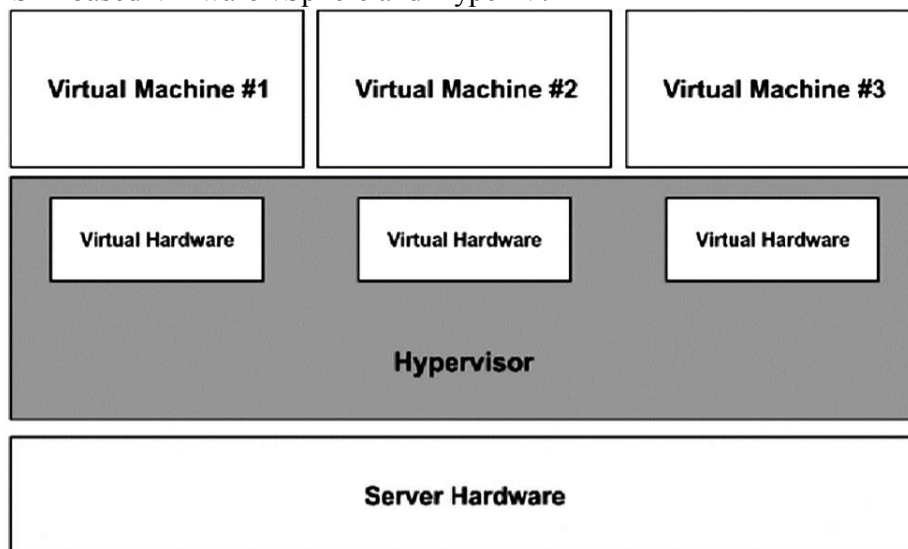
Figure 1.14 Hardware Virtualization
