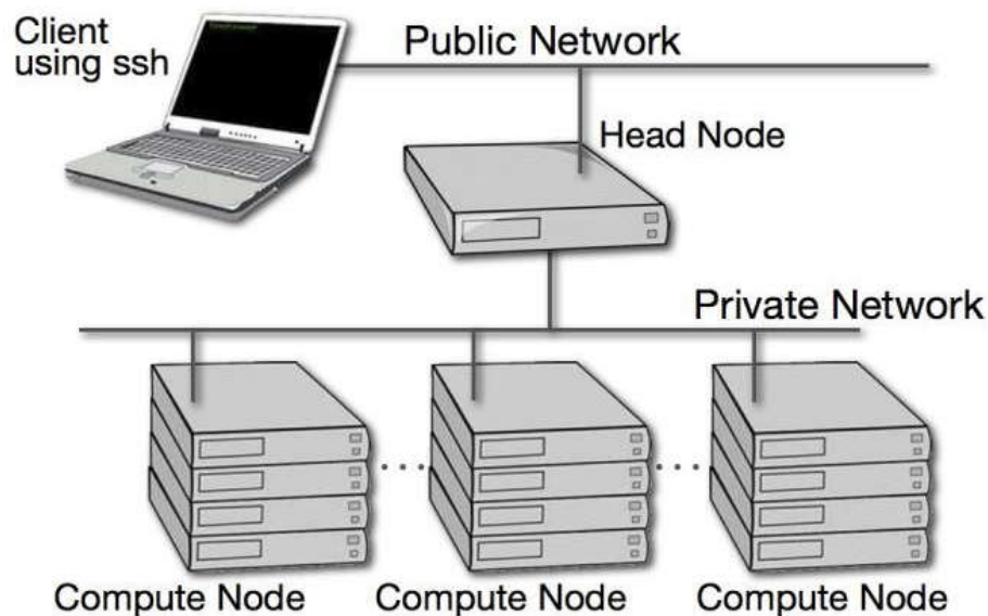
Figure 1.12 Cluster computing
