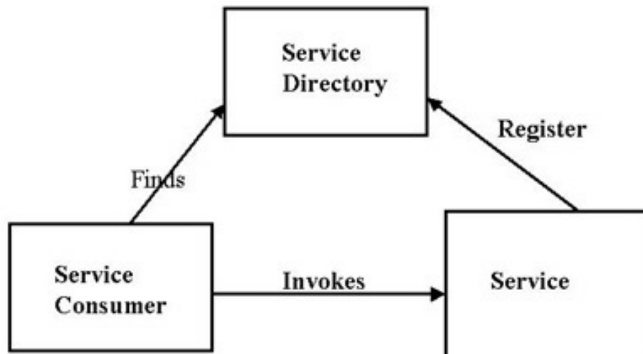
Figure 1.17 Service-oriented Architecture
