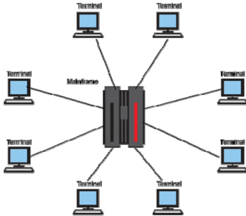
Figure 1.11 Mainframes
