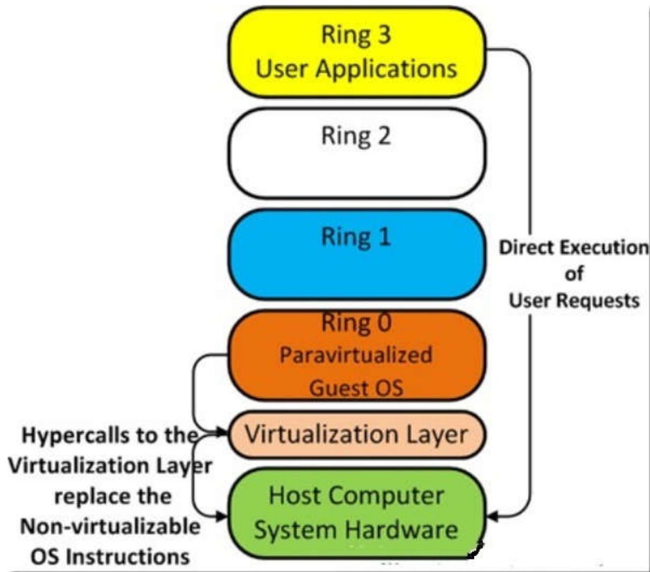
FIGURE 3.13 Hypercalls to virtualization in Paravirtualization
