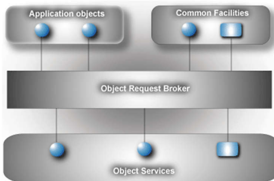
Figure 2.23 Common object request broker architecture (CORBA)
