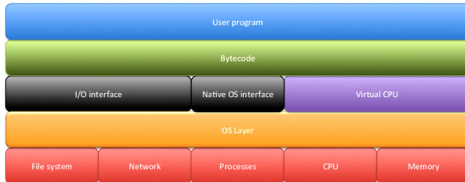
Figure 1.15 process virtual machine design Reference from “Mastering Cloud Computing Foundations and Applications Programming” by Rajkumar Buyya)
