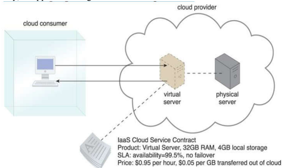
Fig 4.10 cloud customer is using a virtual server within an IaaS atmosphere. cloud consumers are delivered with a range of contractual guarantees by the cloud provider, relating to physiognomies such as capacity, performance, and availability.
