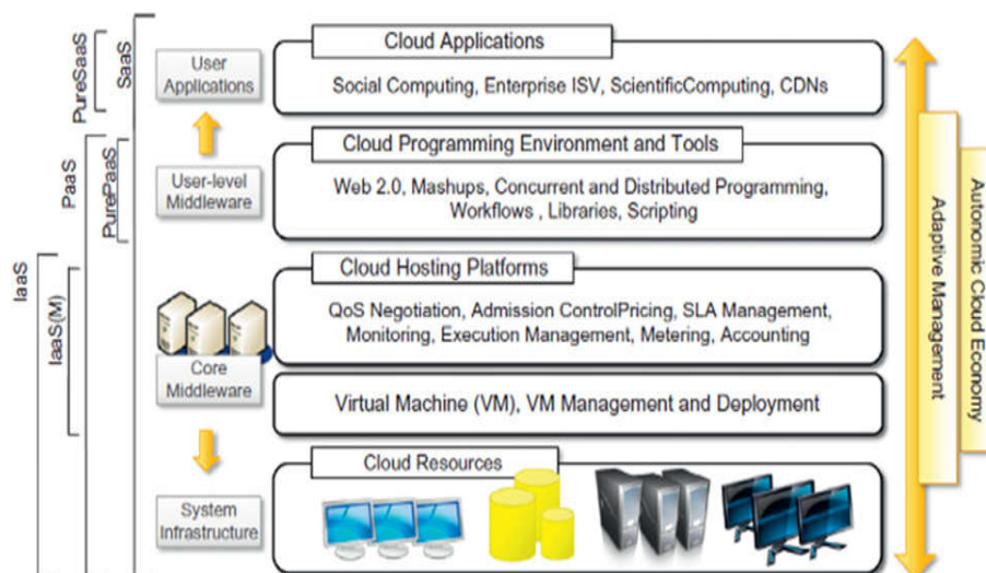
Figure 4.1 The cloud computing architecture (Reference :Cloud Computing(Concepts, Technology & Architecture) by Thomas Erl,Zaigham Mahmood, and Ricardo Puttini)
