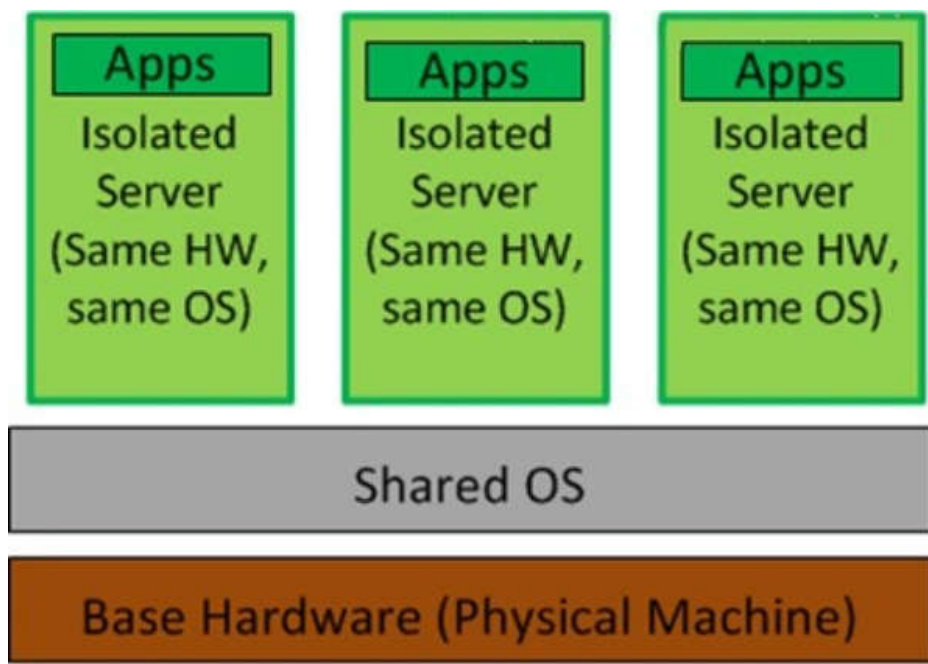
FIGURE 3.14 Operating system-level virtualization
