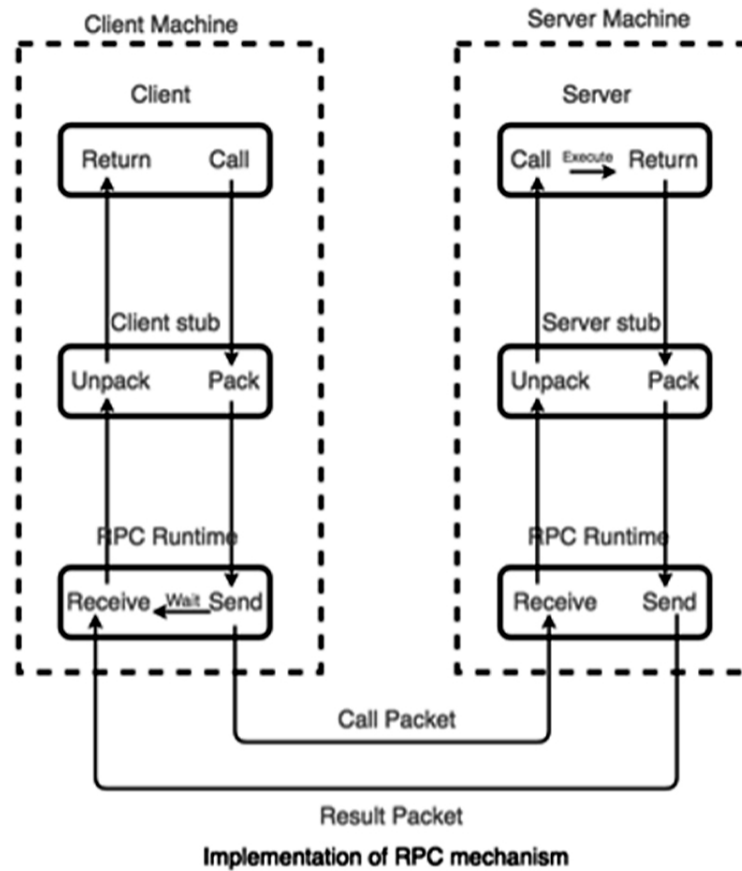
Figure 2.22 Working of Remote Procedure Call
