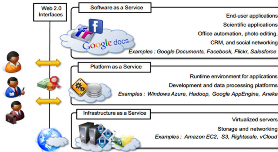
Figure 1.6 The Cloud Computing Reference Model. Reference from “Mastering Cloud Computing Foundations and Applications Programming” by Rajkumar Buyya)
