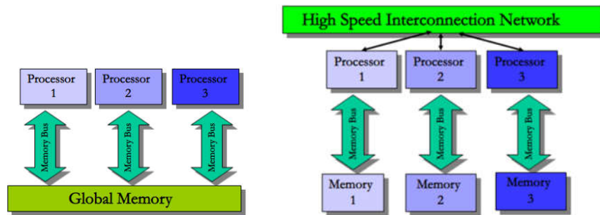
Figure 2.9 shared (left) and distributed (right) memory MIMD architecture.
