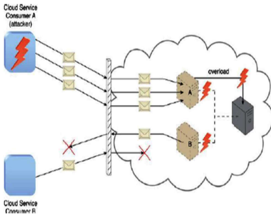
Figure 5.10 Cloud service consumer A sends multiple message to a cloud service(not shown) hosted on virtual server A. This overloads the capacity of the underlying physical server, which causes outages with virtual servers A and B. As a result legitimate cloud service consumers, such as cloud service consumer B, become unable to communicate with any cloud services hosted on virtual servers A and B.
