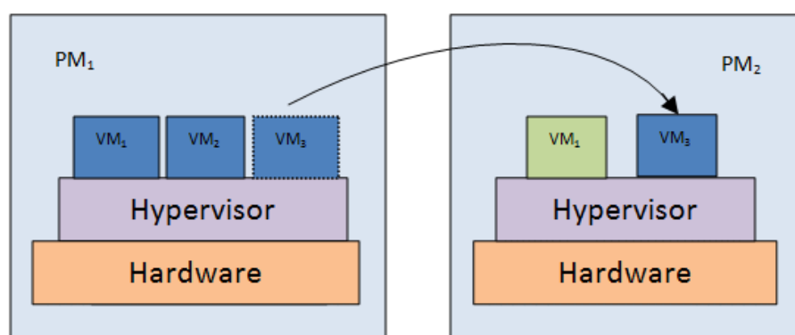
FIGURE 3.16 virtual machine migration
