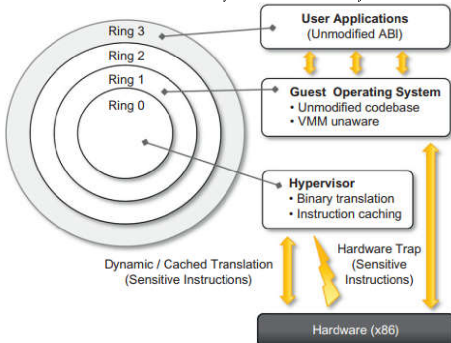
FIGURE 3.18 A full virtualization reference model. (Reference from “Mastering Cloud Computing Foundations and Applications Programming” by Rajkumar Buyya)
