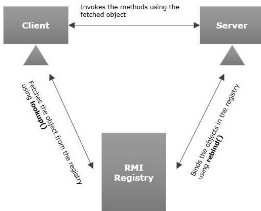
Figure 2.26 RMI program works
