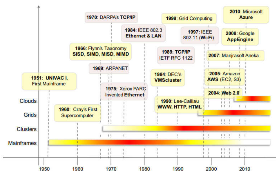
Figure 1.10: The evolution of distributed computing technologies, 1950s-2010s. Reference from “Mastering Cloud Computing Foundations and Applications Programming” by Rajkumar Buyya)
