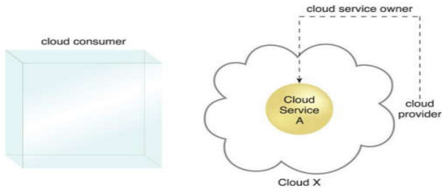
Figure 4.3 A cloud provider becomes a cloud service owner if it deploys its own cloud service, typically for other cloud consumers to use.
