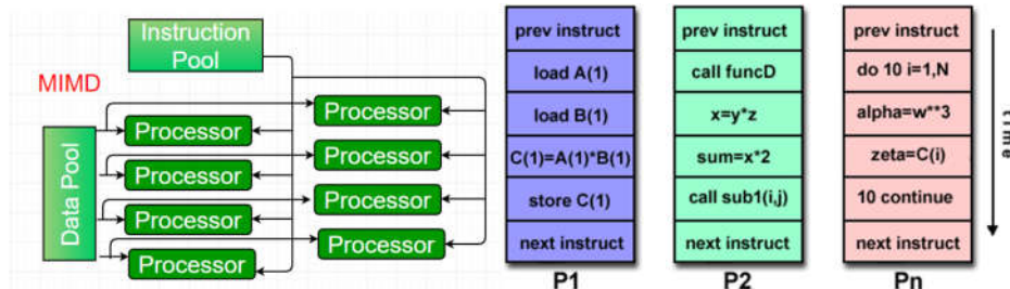
Figure 2.8 Multiple-instructions, multiple-data (MIMD) architecture.
