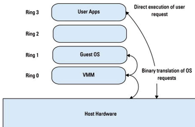
FIGURE 3.11 Full Virtualization
