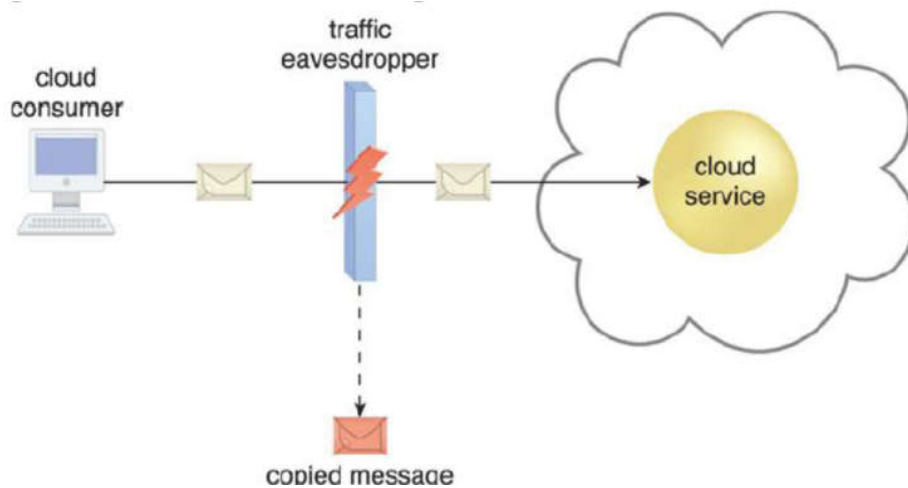
Figure 5.8 An externally positioned malicious service agents carries out a traffic eavesdropping attack by intercepting a message sent by the cloud service consumer to the cloud service. The service agent makes an unauthorized copy of the message before it is sent along its original path to the cloud service.
