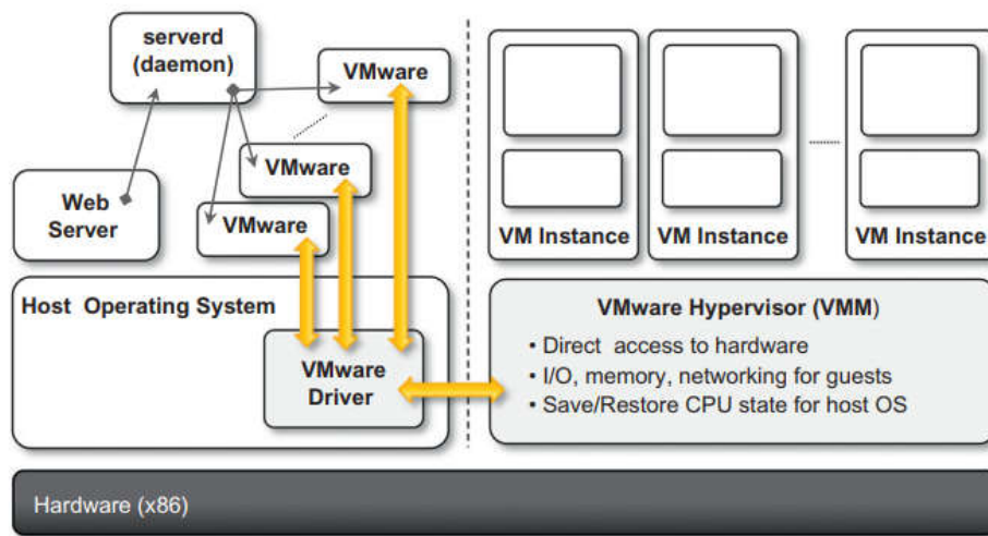
FIGURE 3.20 VMware GSX server architecture. (Reference from “Mastering Cloud Computing Foundations and Applications Programming” byRajkumar Buyya)
