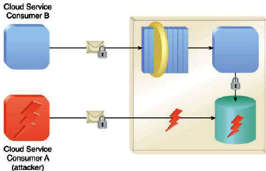
Figure 5.11 Cloud service consumer A gains access to a database that was implemented under the assumption that it would only be accessed through a web service with a published service contract (as per cloud service consumer B)(Reference :Cloud Computing(Concepts, Technology & Architecture) by Thomas Erl,Zaigham Mahmood, and Ricardo Puttini)
