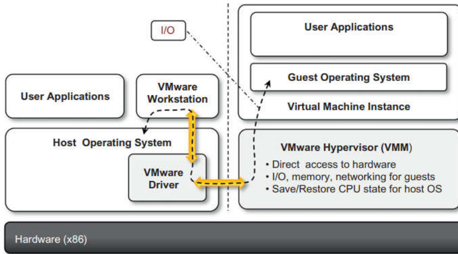
FIGURE 3.19 VMware workstation architecture. (Reference from “Mastering Cloud Computing Foundations and Applications Programming” byRajkumar Buyya)
