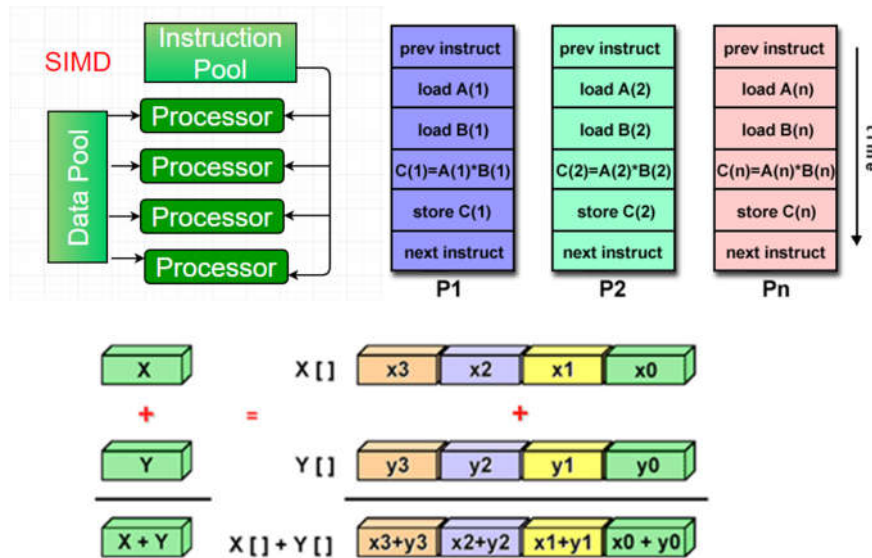
Figure 2.6 : Single-instruction, multiple-data (SIMD) architecture.
