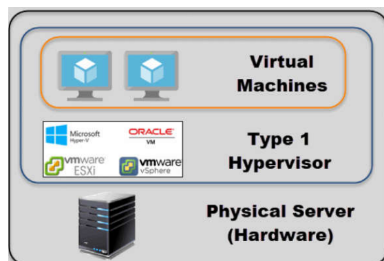
FIGURE 3.7 Type 1 Hypervisor
