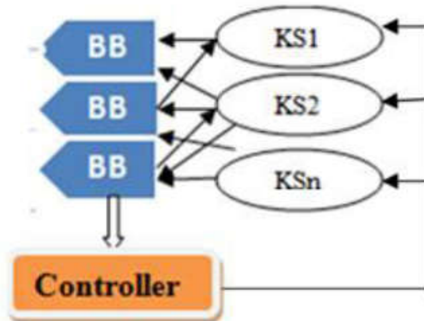
Figure 2.15 Blackboard architecture
