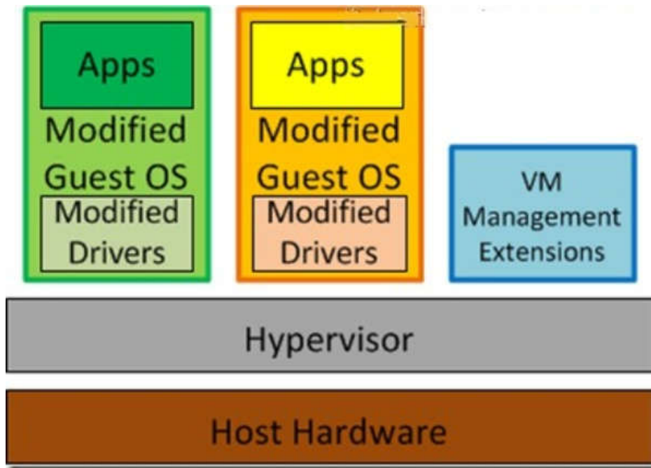
FIGURE 3.12 Paravirtualization
