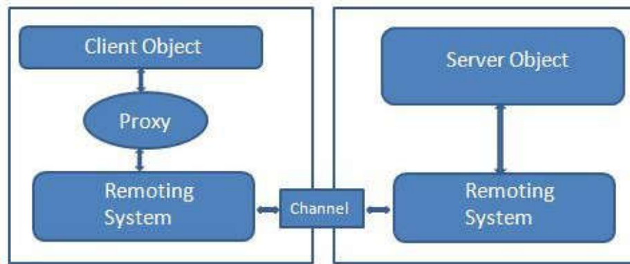
Figure 2.27 .NET remoting Framework
