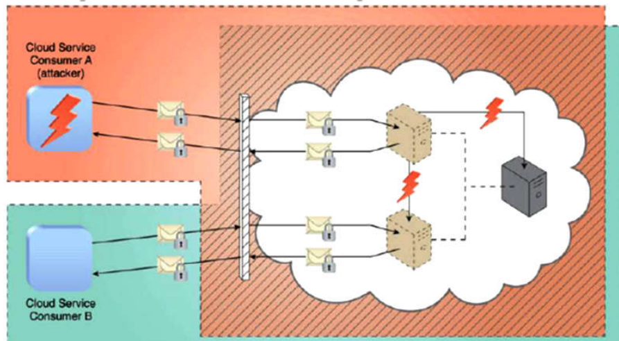
Figure 5.13 illustrates an example in which two cloud service consumers share virtual servers hosted by the same physical server and, resultantly, their respective trust boundaries overlap.
