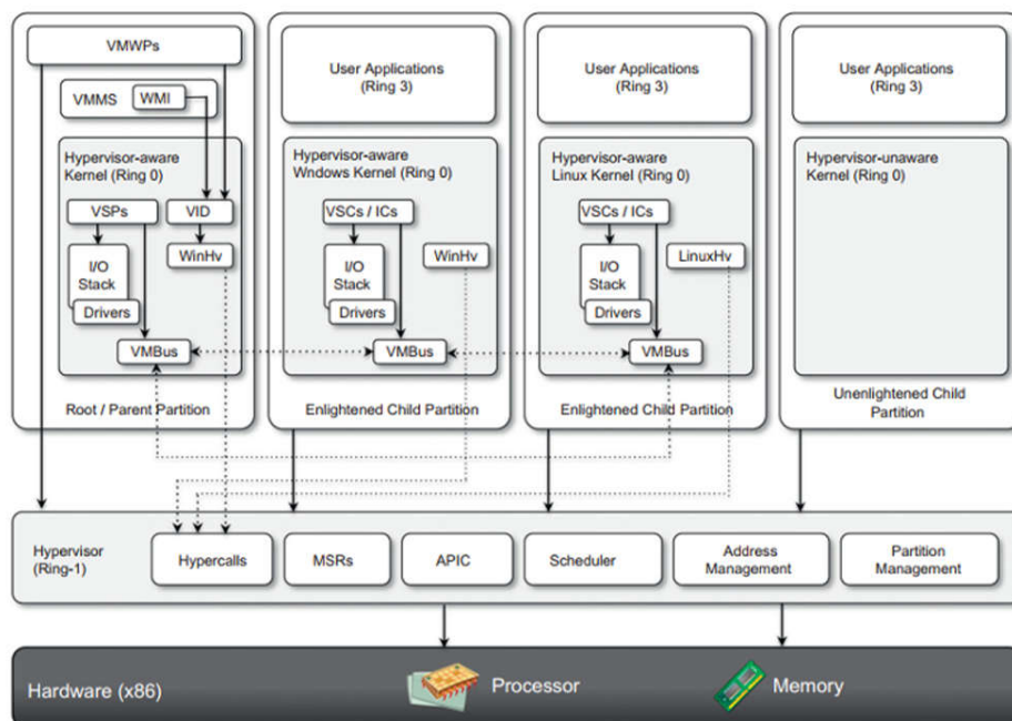
FIGURE 3.22 Microsoft Hyper-V architecture (Reference from “Mastering Cloud Computing Foundations and Applications Programming” by Rajkumar Buyya)
