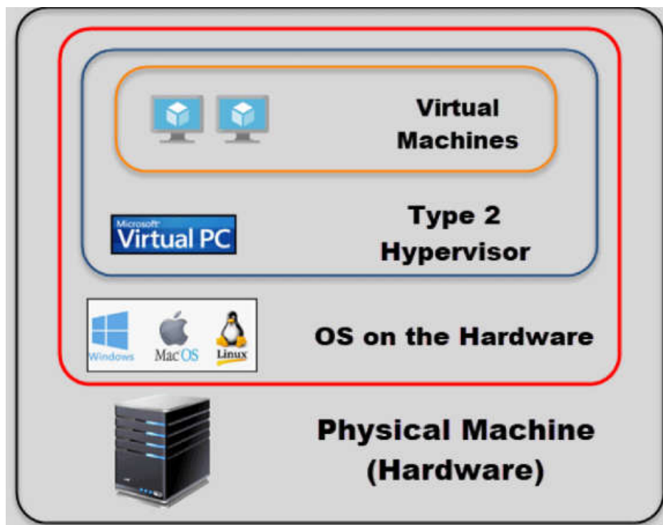
FIGURE 3.8 Type 2 Hypervisor
