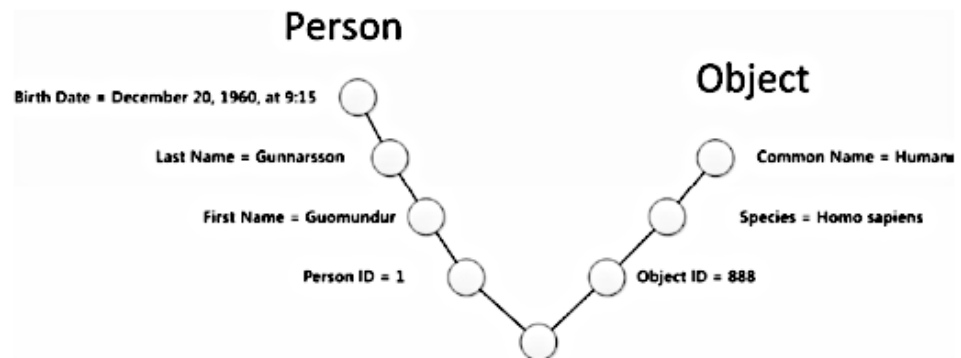
Figure 3b.4 Sun model for the PersonIsSpecies fact
