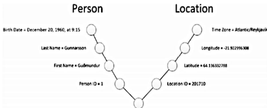
Figure 3b.5 Sun model for PersonAtLocation fact
