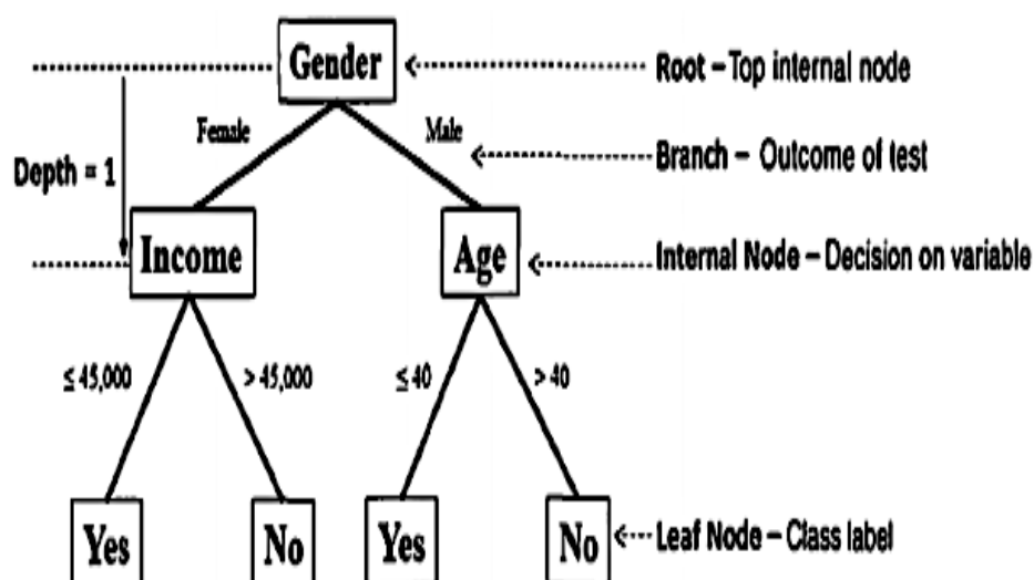
Figure 3b.10 Decision Tree
