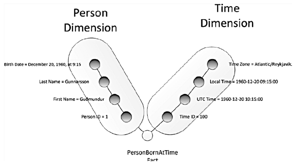
Figure 3b.3 Person-to-Time sun model (explained)
