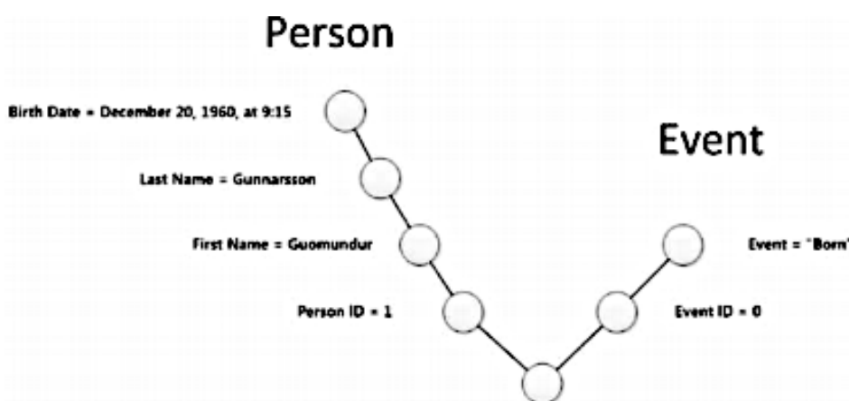
Figure 3b.6 Sun model for PersonBorn fact
