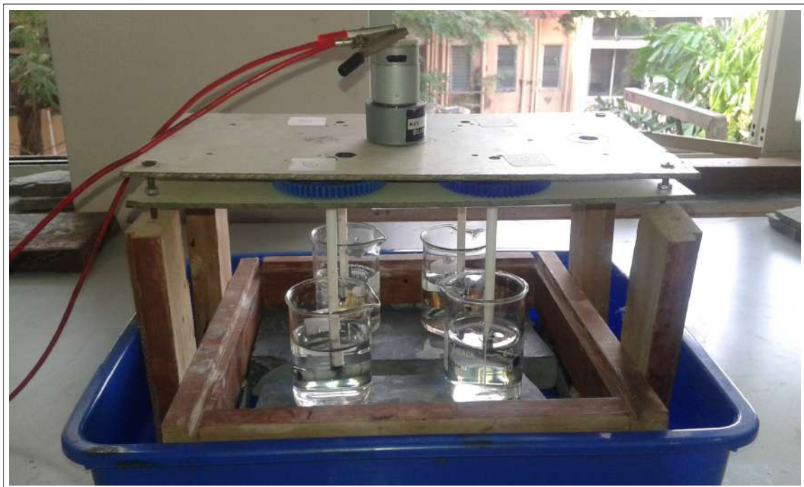
Indigenously developed in-house magnetic stirrer
