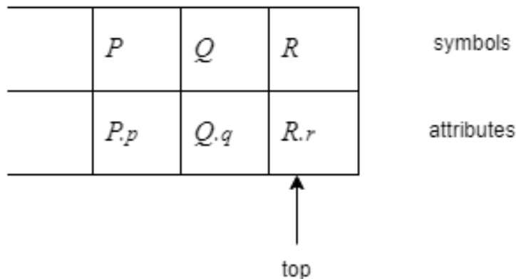
Fig 3.6 Parser stack
