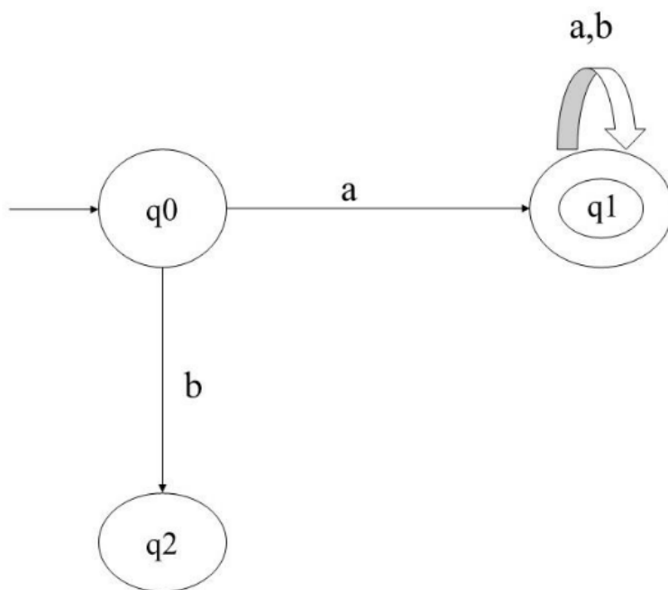
Figure 7. DFA
