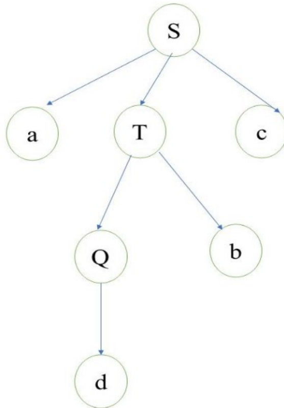
Figure 19. Parse tree
