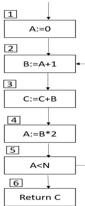
Fig 3.12 flow graph
