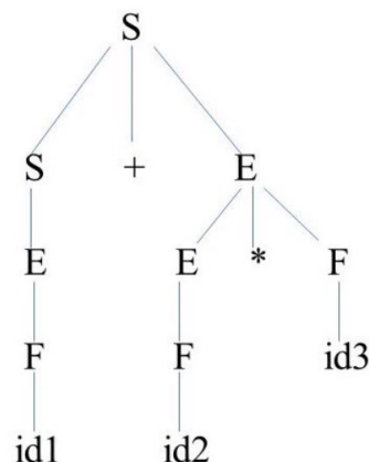
Figure 15. Parse tree
