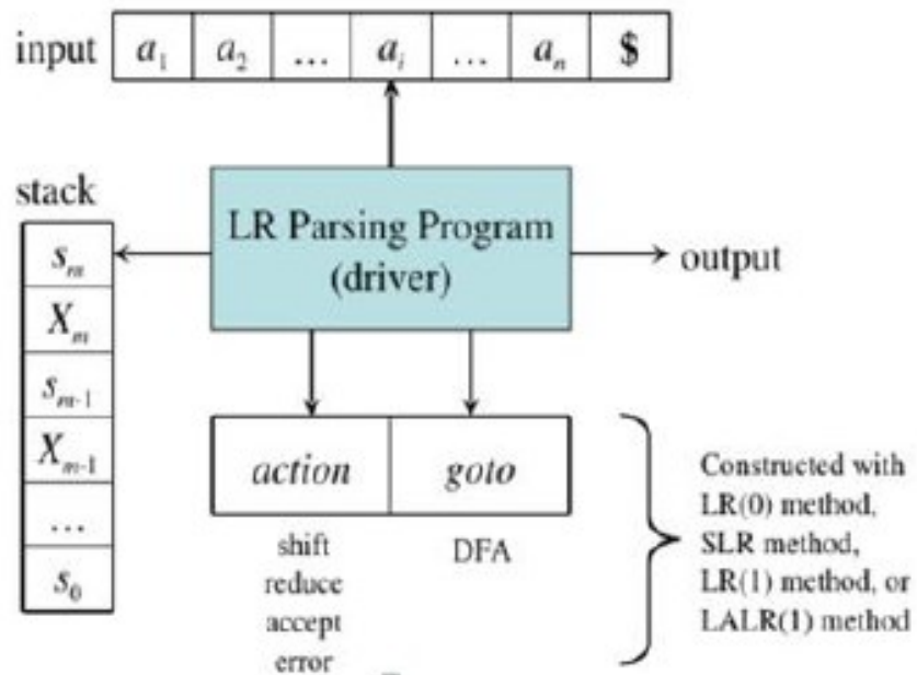
Above fig. – Model of an LR Parser.
