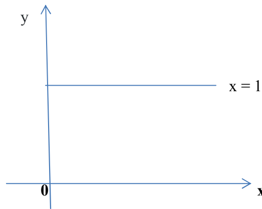
Figure 1 The Heaviside step function H(x)
