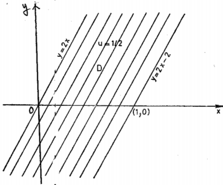
Fig 1.3 The domain D when the Cauchy data is u(x, 0) = 1/2 for 0 \leq x \leq 1 .
