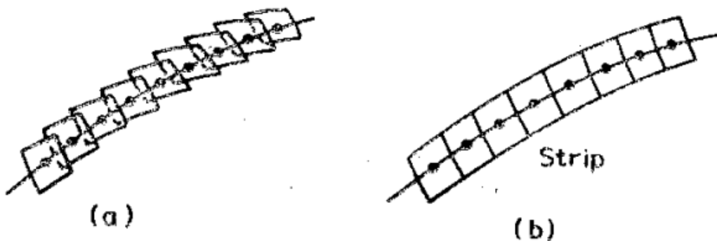
Fig 1.6 . Any set of five functions does not form a strip as in (a). The planes must be tangent to the curve and their normal should vary continuously (b).
