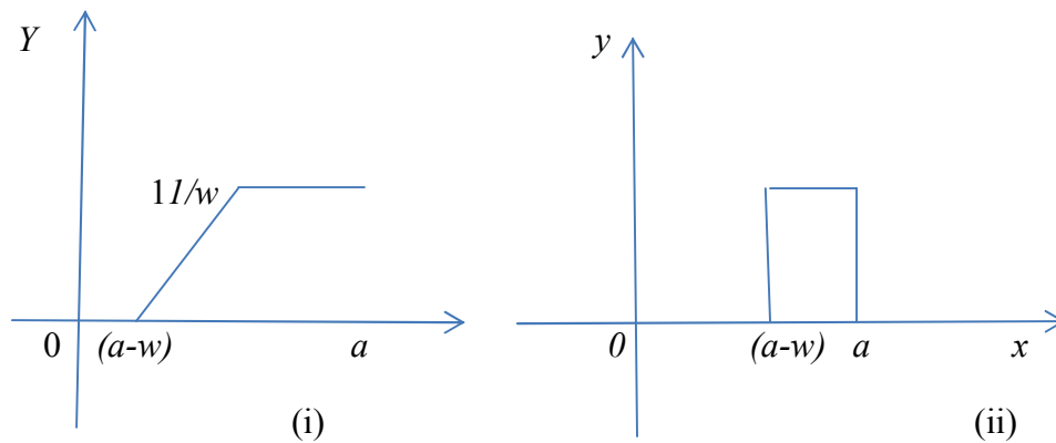
Figure 3 Ramp approximation to the step function and its derivative
