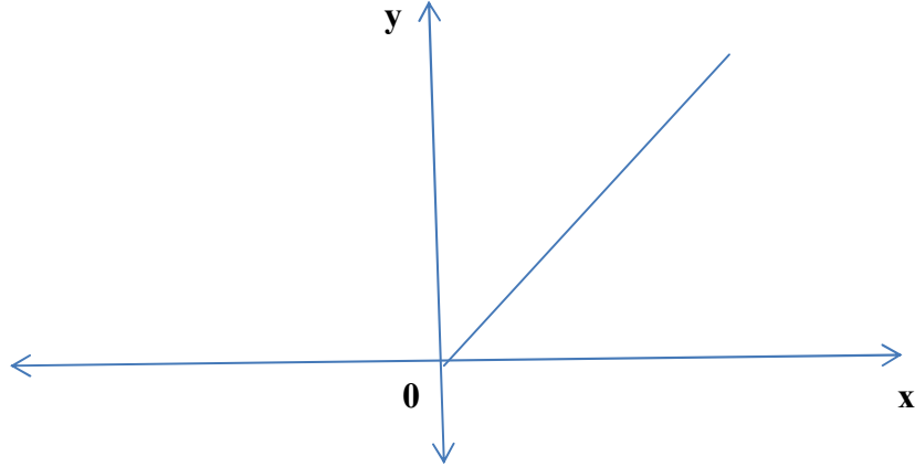
Figure 2 The ramp function
