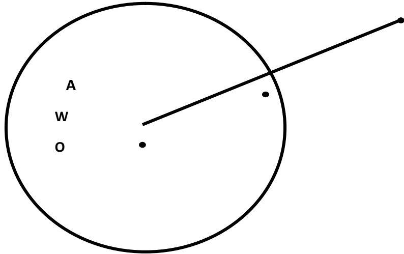
Fig. w and \frac{R^2}{\bar{w}} are inverse point with respect to C: |z| = R
