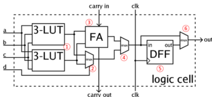
Figure 1.6: A simplified CLB: The four-input LUT is formed from two three-input units
