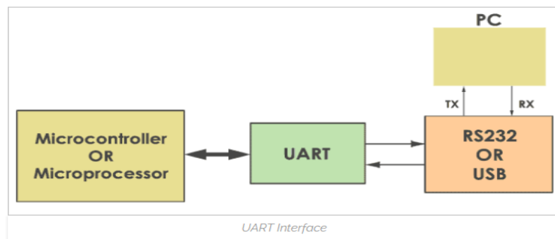
Figure 4.2 UART interface
