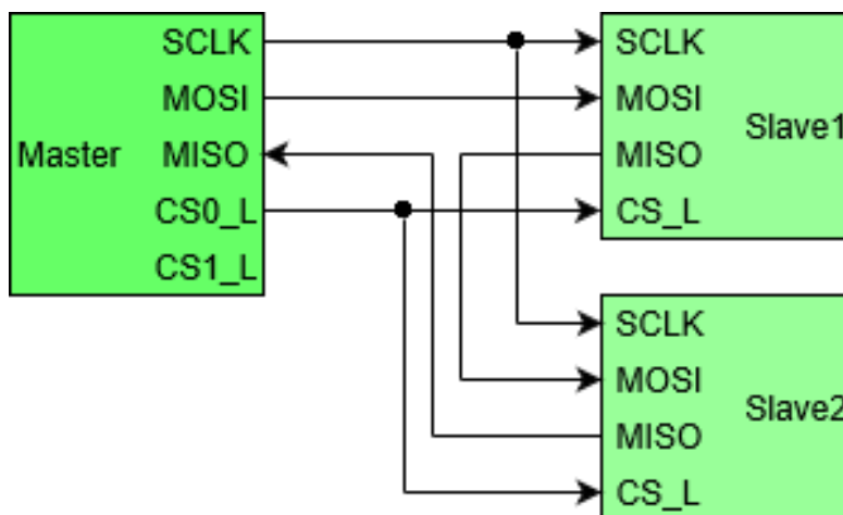
Figure 1.8 SPI Bus – Daisy Chain Topology
