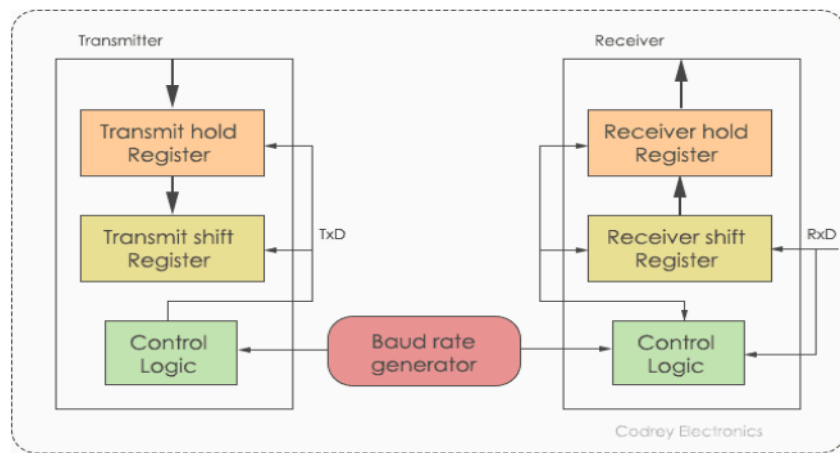
Figure 4.3 UART block diagram
