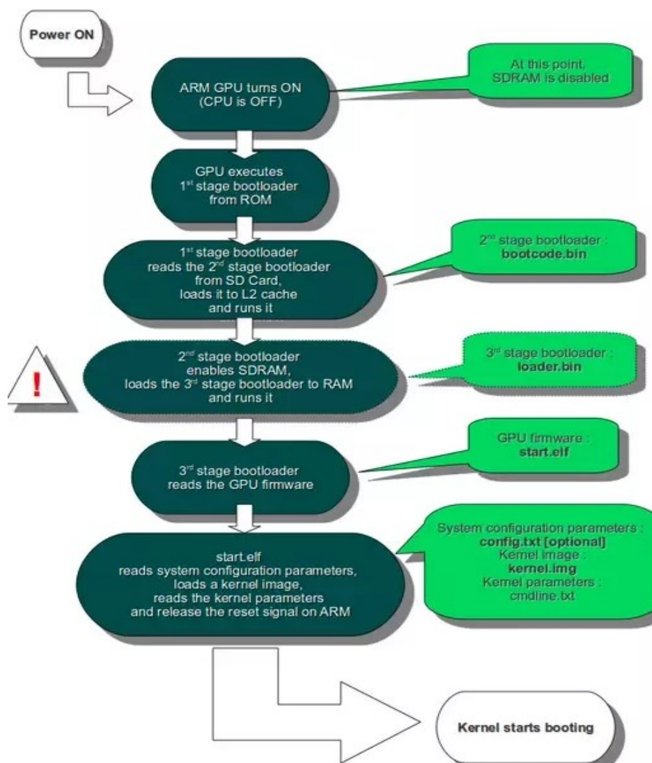
Figure 1.46 Flow process of boot sequence configuration
