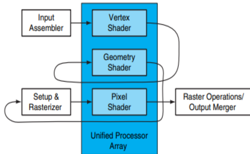
Figure 1.8 Logical pipeline mapped to physical processors. On the array of unified processors, the programmable shader stages run, and the logical graphics pipeline dataflow recirculates via the processors.
