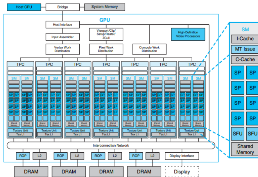
Figure 1.9 Basic unified GPU architecture
