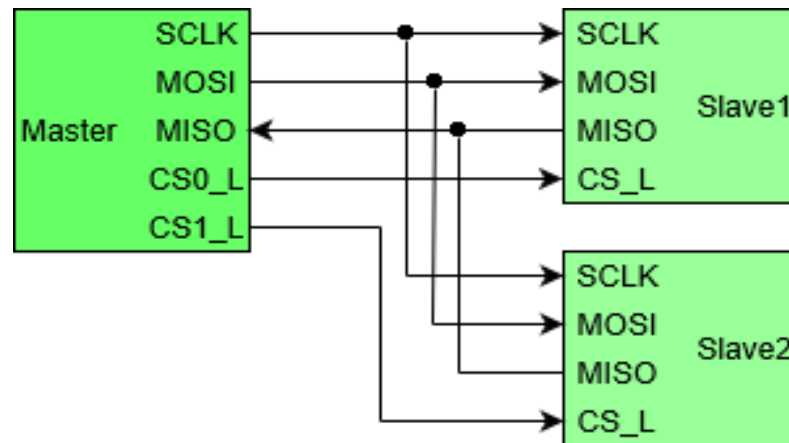
Figure 1.9 SPI Bus – Star Topology
