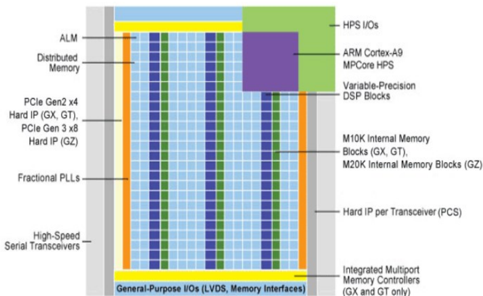
Figure 1.3 An overview of FPGA
