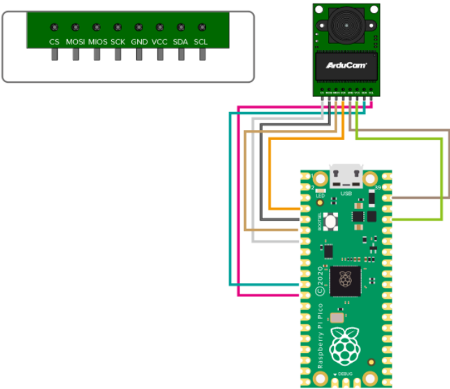
Connect SPI Camera to Pico
