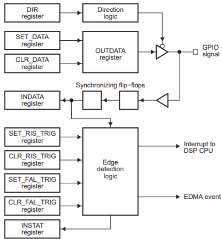
Figure 1.5 GPIO peripheral block diagram
