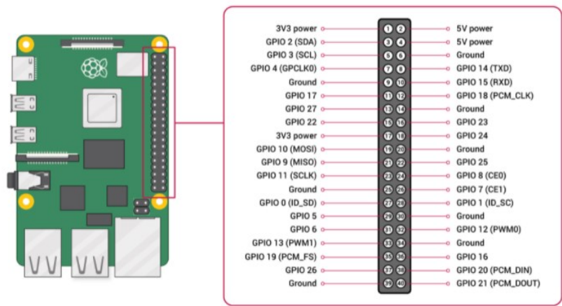
Figure 1.6 Raspberry Pi4 GPIO pin header
