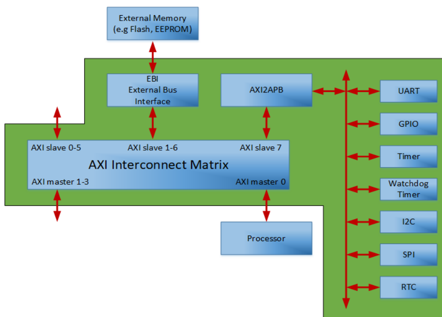
Figure 1.1 Building blocks of SoC
