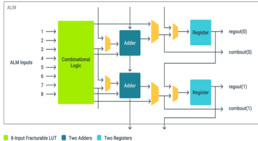
Figure 1.4 Adaptive Logic Module of an Altera/Intel FPGA
