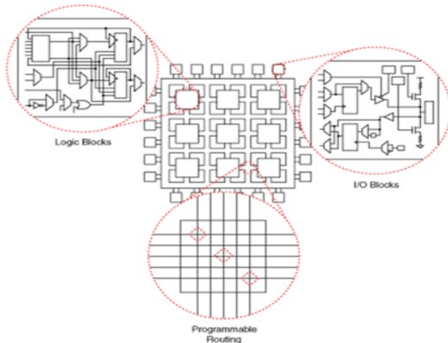
Figure 1.5: The fundamental FPGA architecture
