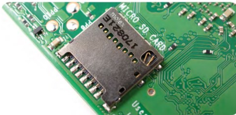
Figure 1.38 The Raspberry Pi's microSD card connector
