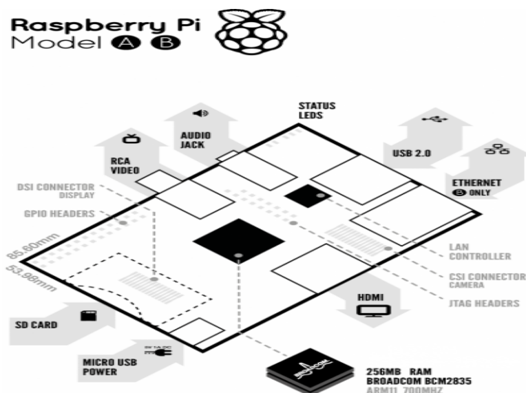
Figure 1.45 Raspberry Pi with the Broadcom BCM2835 SoC
