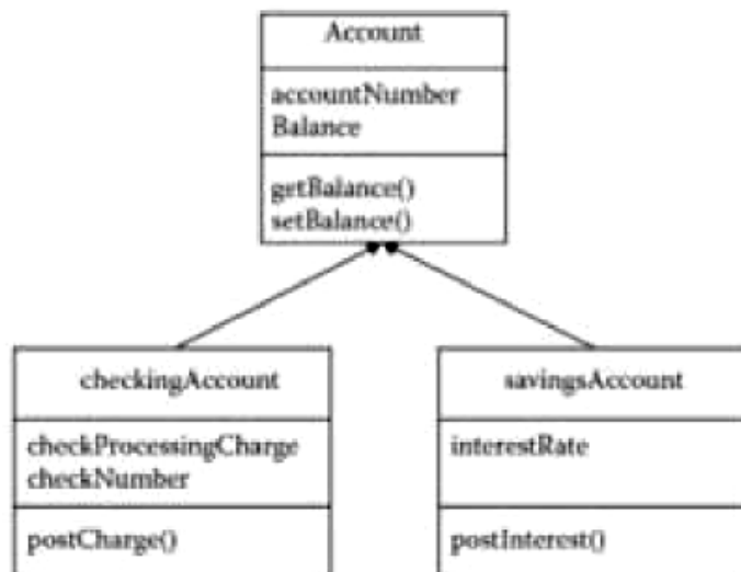
Figure 7.3.1 UML inheritance
