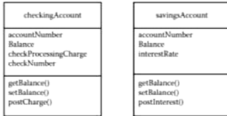
Figure 7.3.2 Flattened classes
