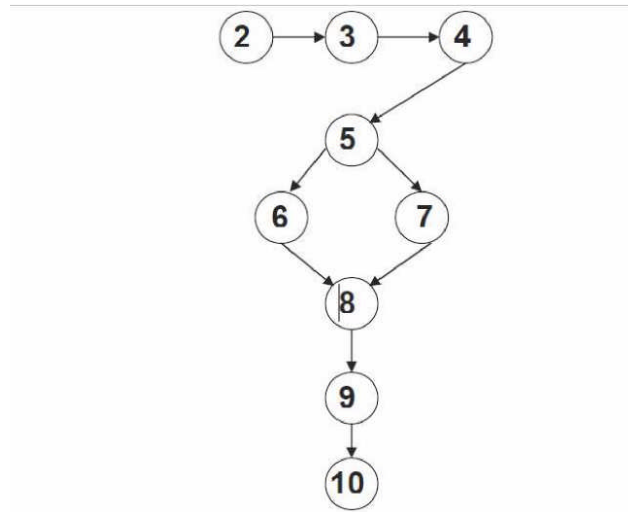
Figure 1.2 A program graph of the simple subtraction program
