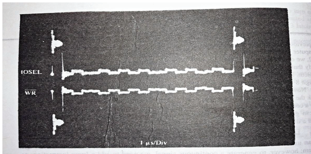
Figure 4.14 :- Timing Signals of Diagnostic Routine
