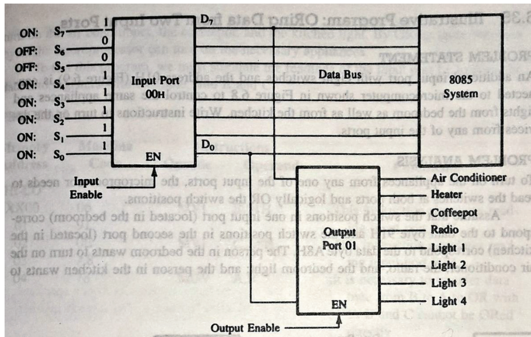
Figure 6.8:- Input Port To Control Appliances
