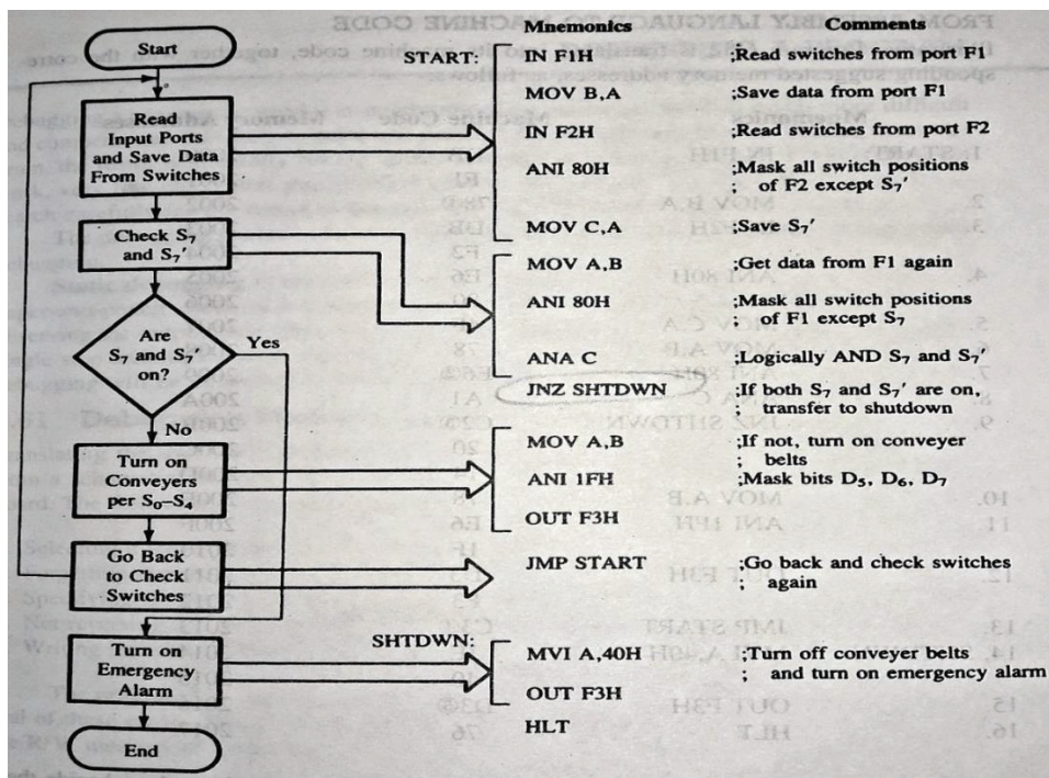
Figure 6.13: Flowchart and Program for Controlling Manufacturing Processes
