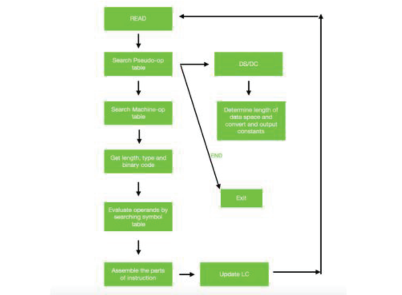
Fig. 2 - Flow chart of how assembly work
