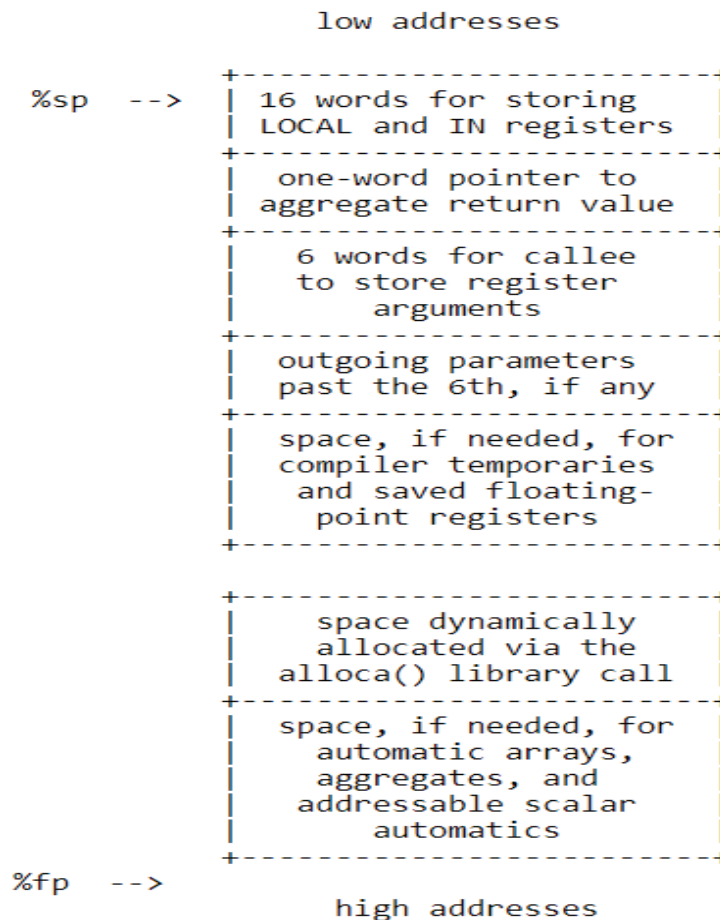
Figure 2.3: Stack Frame Contents
