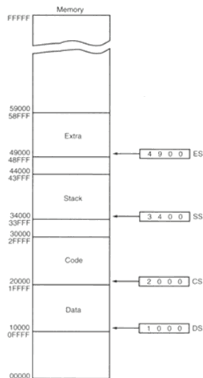
Figure 3.2: A memory system showing the placement of four memory segments
