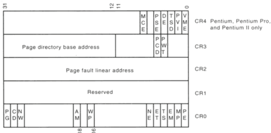
Figure 3.4: The control register structure of the microprocessor
