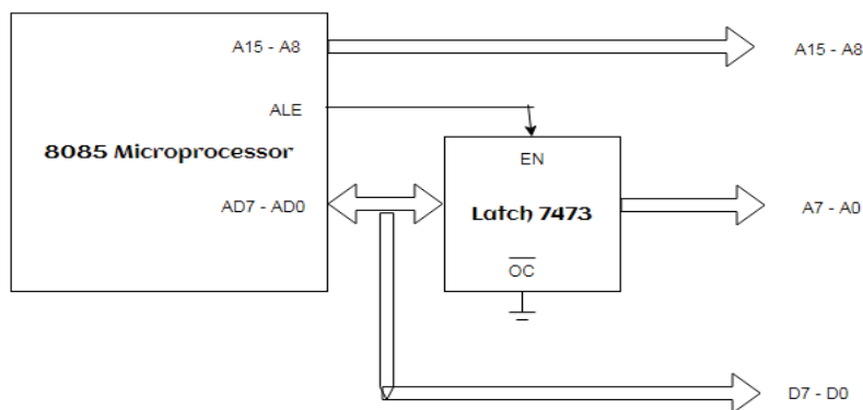
Figure 3.3 – Latching the multiplexed bus
