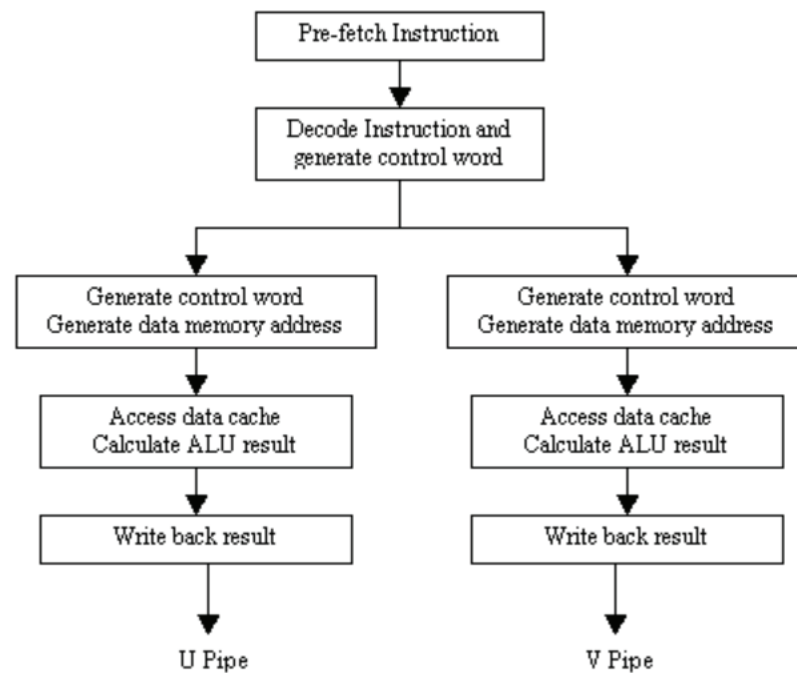
Figure 1.3: Pentium Pipeline Stages
