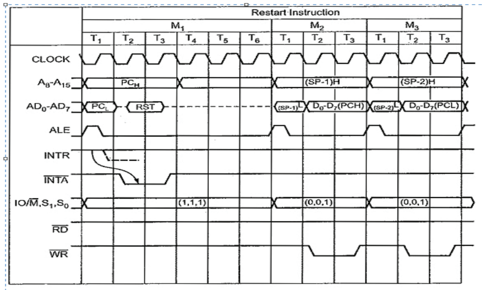
Figure 13.2 – \overline{INTA} and RST 5 Timing Diagram
