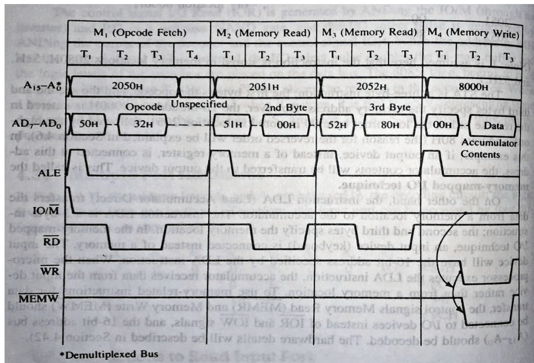
Figure 4.12 :- Timing for Execution of the Instruction STA 8000H
