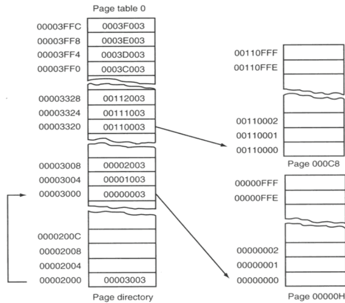
Figure 3.7: The page directory, page table 0, and two memory pages
