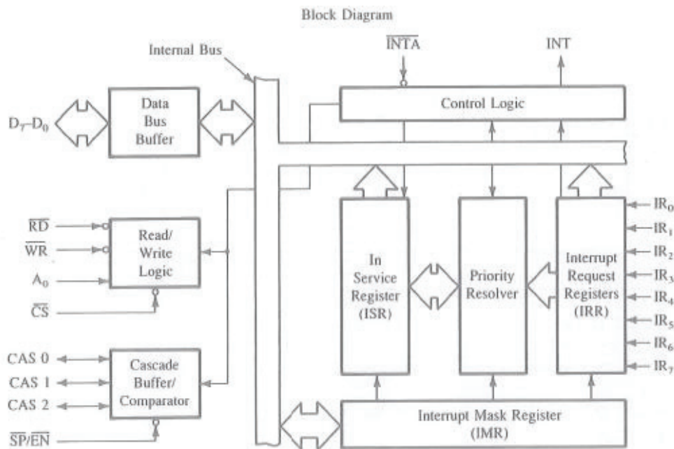
Figure 13.6 – 8259A Architecture Diagram
