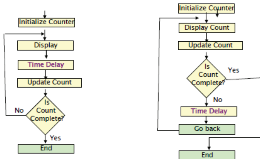
Fig 5 Variations of Counter Flow chart
