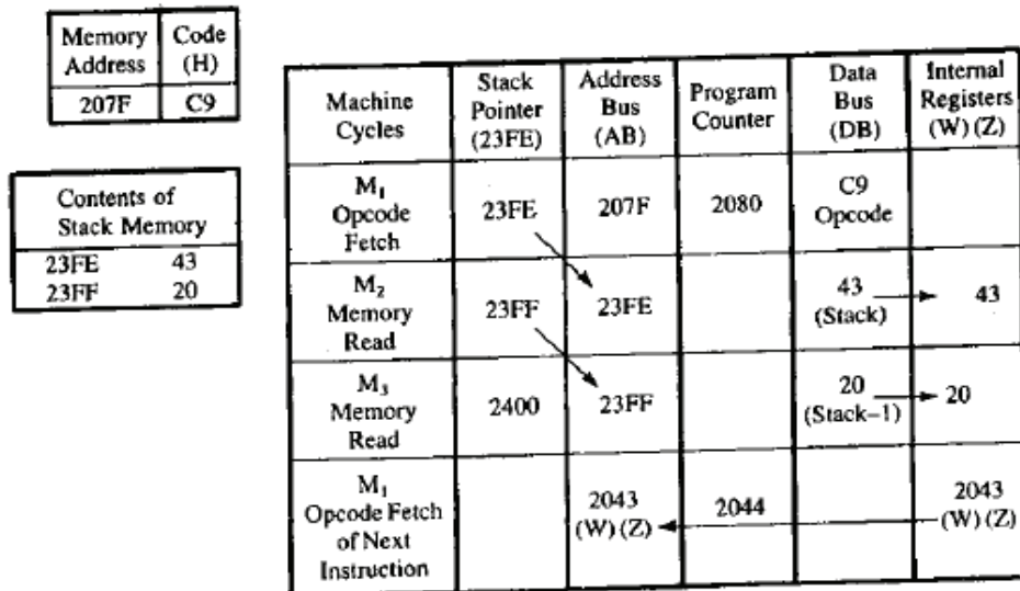
Data Transfer During the Execution of the RET Instruction
