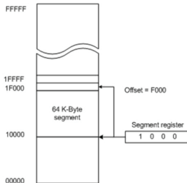
Figure 3.1: The real mode memory addressing scheme
