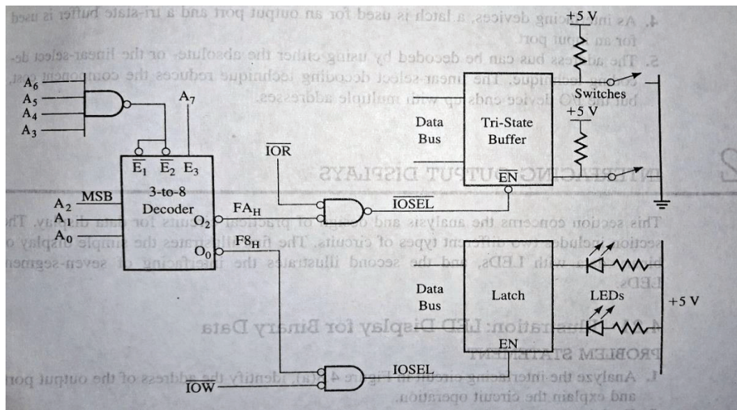
Figure 4.7 :- Address Decoding Using 3-to-8 Decoder
