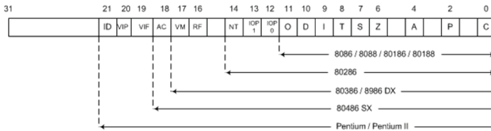
Figure 2.2: EFLAGS Register
