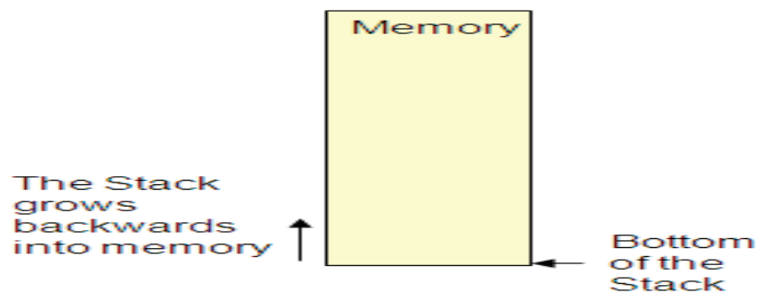
Fig 1 Stack Structure
