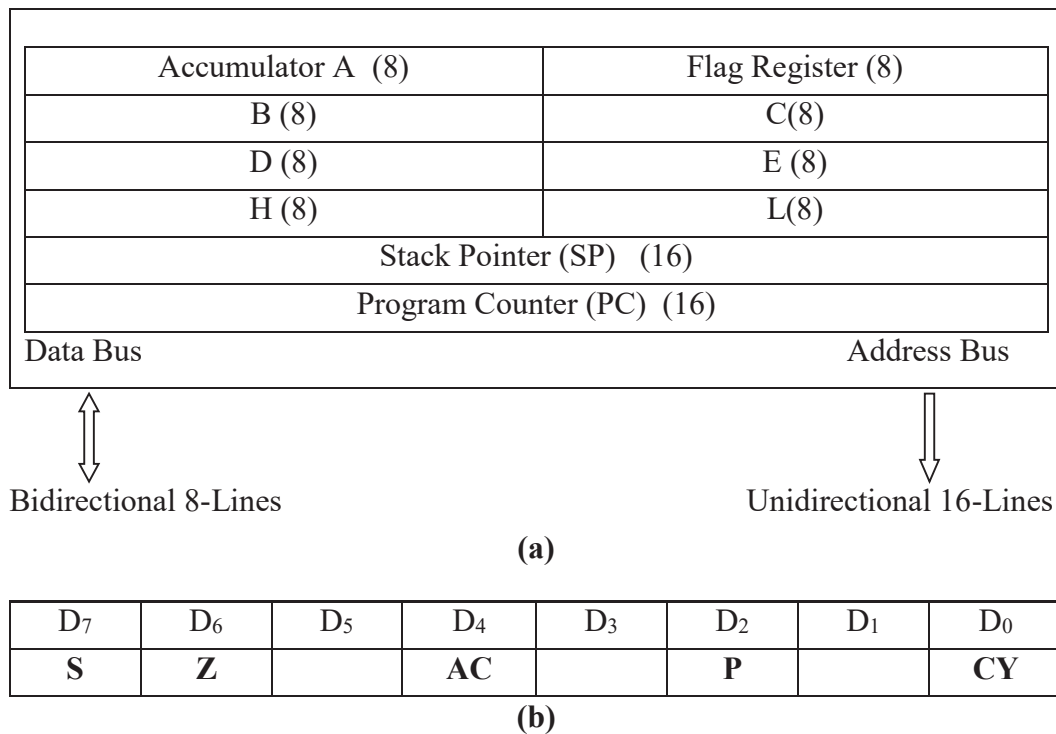
Figure 5.1: 8085 Programming Model (a) and Flag Register (b)
