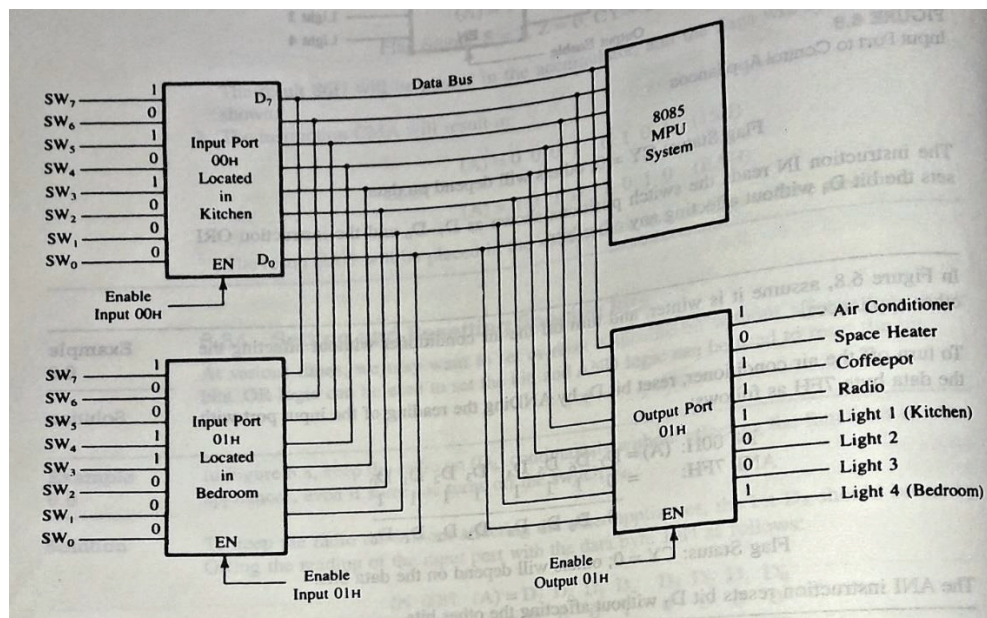
Figure 6.9 Two Input Ports to Control Output Devices
