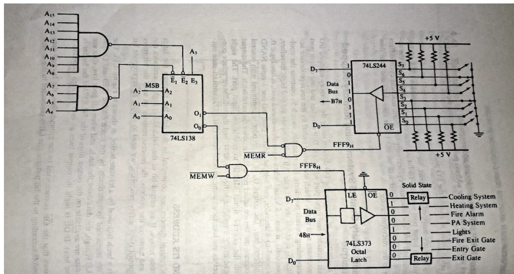
Figure 4.13 :- Memory-Mapped I/O Interfacing
