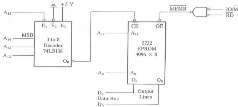
Figure 3.12 – Interfacing 4096 x 8 EPROM Memory
