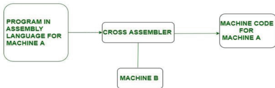
Fig. 4 - Cross Assembler
