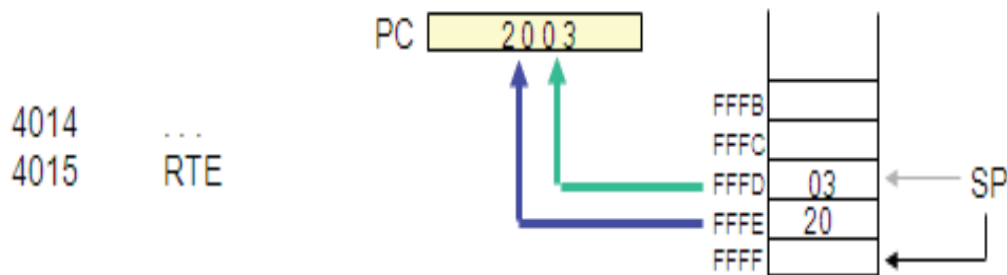
Fig. 6 - RTE Instruction
