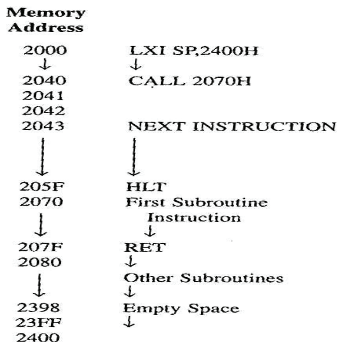
Fig. 7 - Program
