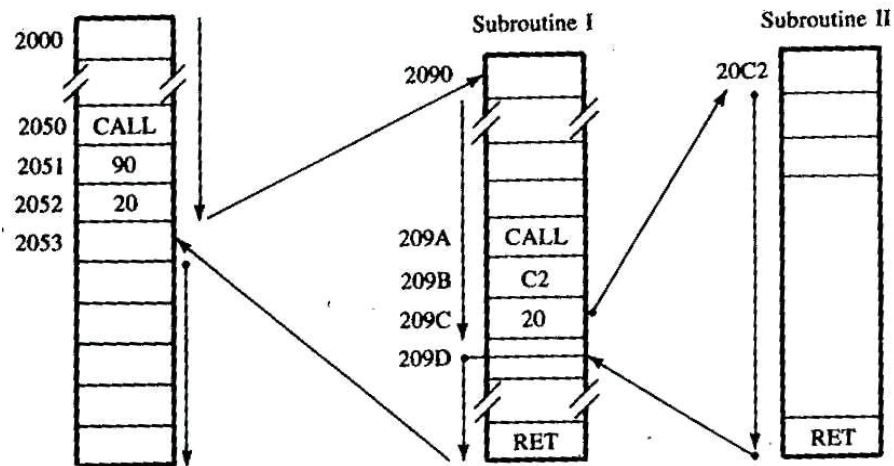
Fig. 15 - Nested Subroutines
