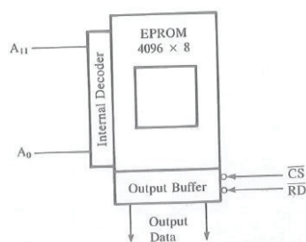
Read Only Memory Chip (4096 x 8)
