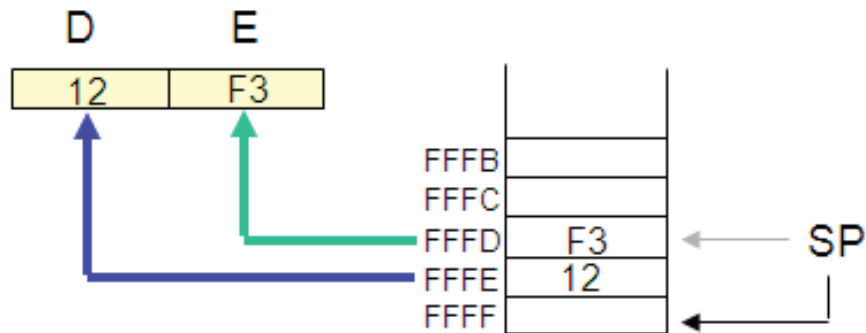
Fig.3 - POP operation on Stack
