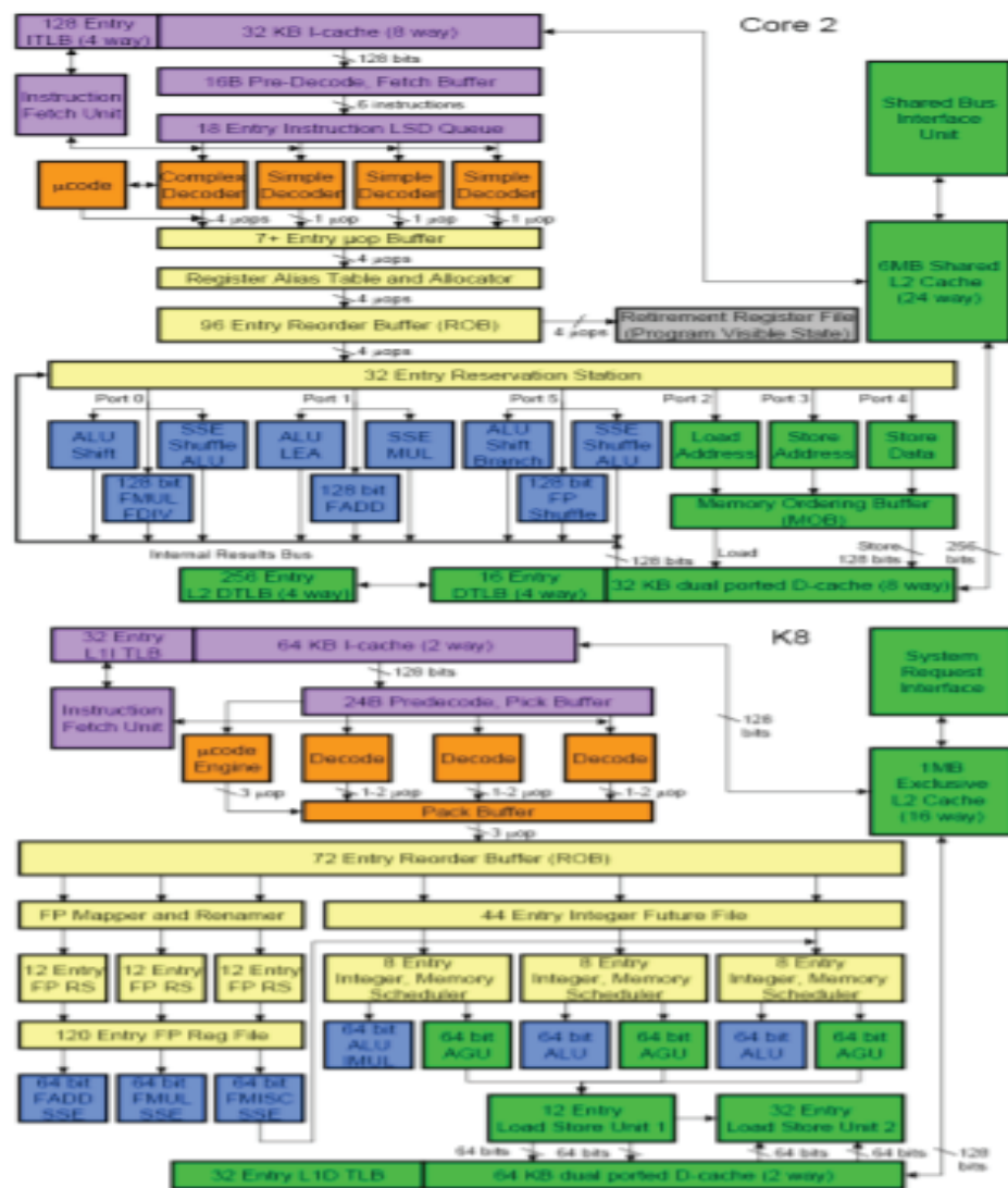
Figure 4.2: Intel Core 2 Microarchitecture
