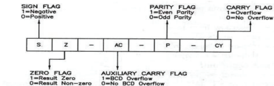
Figure 3.6 – 8085 Flag Register Format
