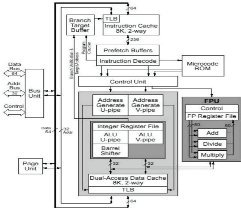
Figure 3.1: The Pentium Architecture
