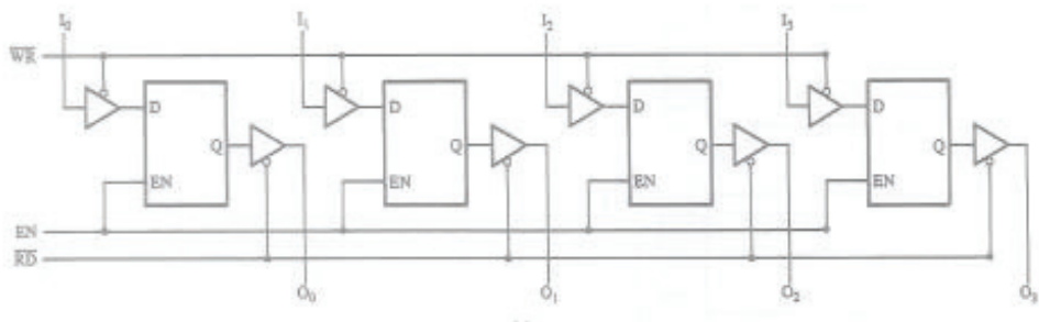
Figure 2.4 – 1 x 4 memory organization
