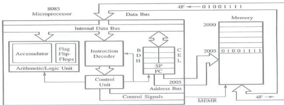
Figure 2.12 – Instruction Fetch Operation
