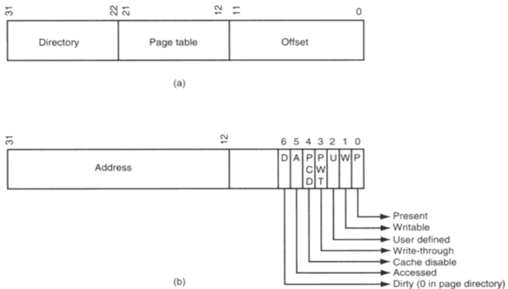
Figure 3.5: The format for the linear address (a) and a page directory or page table entry (b)
