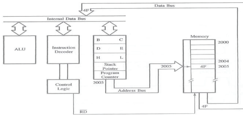
Figure 3.2 – Communication flow of instruction execution
