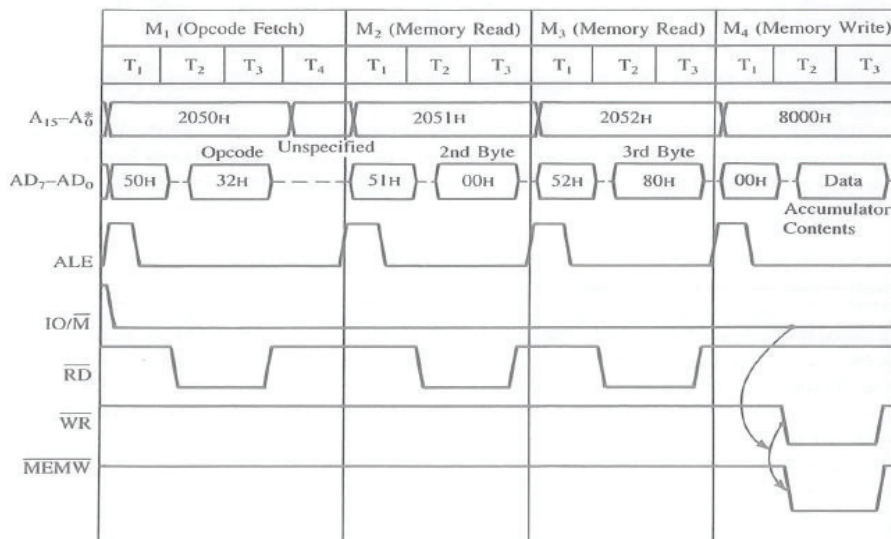
Figure 3.9 – Machine Cycles for the instruction STA 8000H
