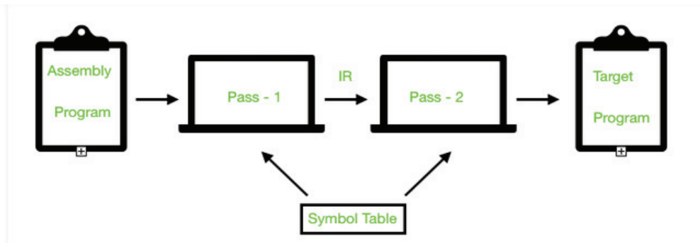
Fig. 3 - As a whole working of assembler
