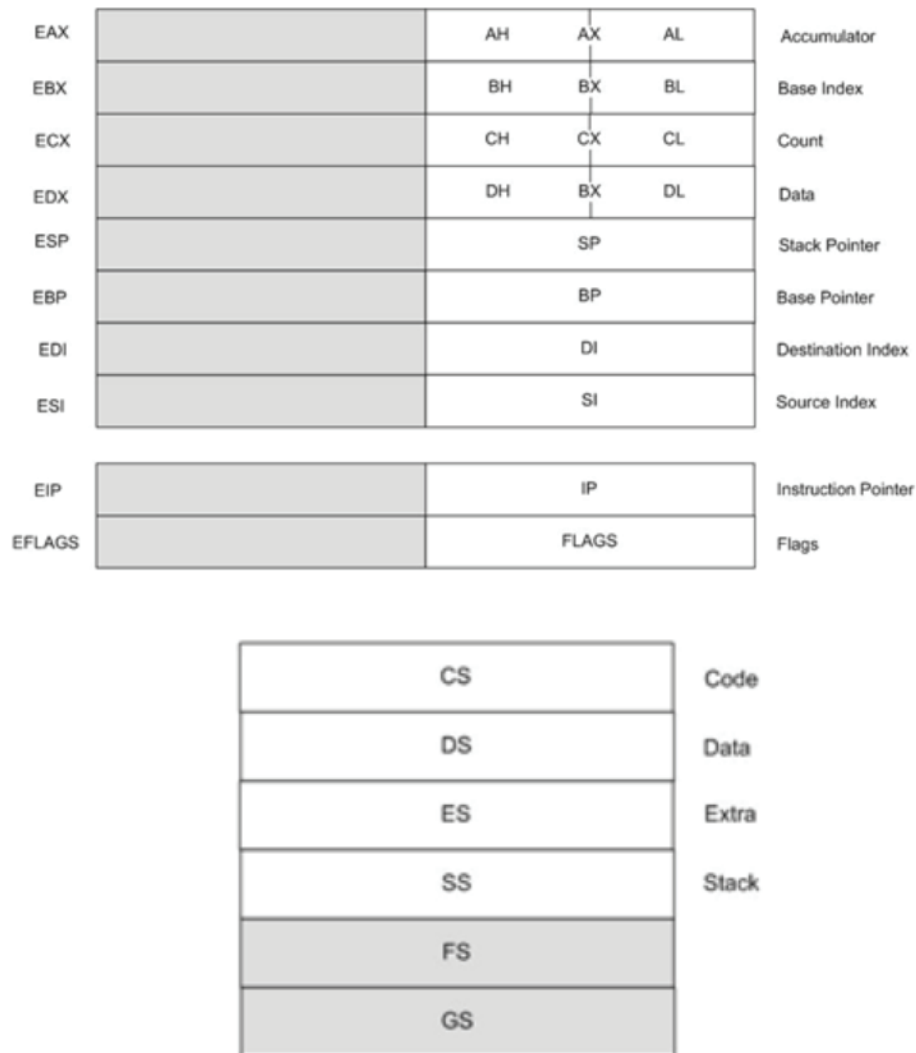
Figure 2.1: The Programming Model of Microprocessor
