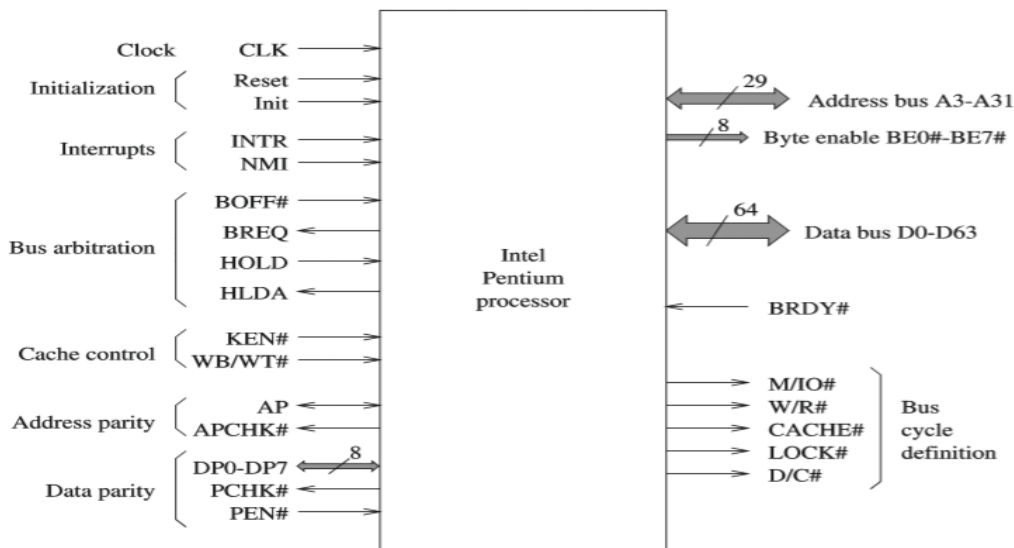
Figure 1.1: Pentium Processor
