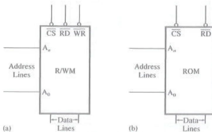
Figure 2.9 – R/W and ROM model
