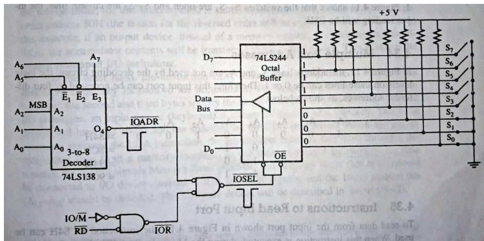
Figure 4.11:- Interfacing DIP Switches
