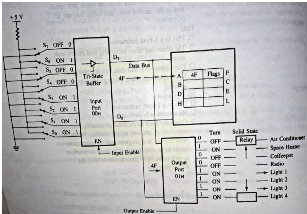
Figure 6.1: Reading Data at Input Port and Sending Data to Output Port
