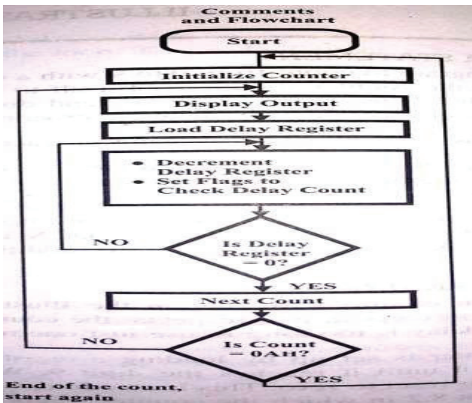
Fig 6 Flow chart Modulo Ten Counter
