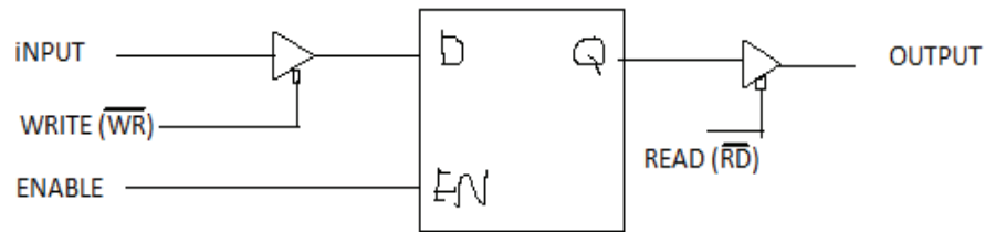
Figure 2.3 – Basic D Latch with Tristate Buffers
