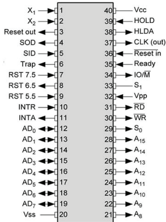
Figure 3.1 – Pin Configuration
