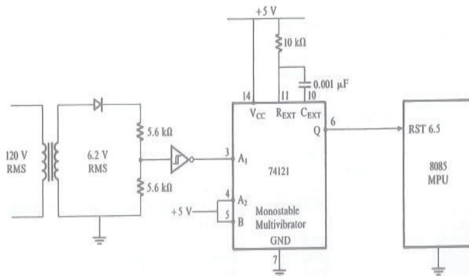
Figure 13.5 – Interrupt Driven Clock
