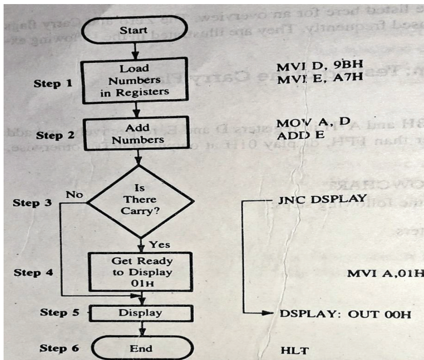
Figure 6.10: Flowchart And Assembly Language Program to Test Carry Flag
