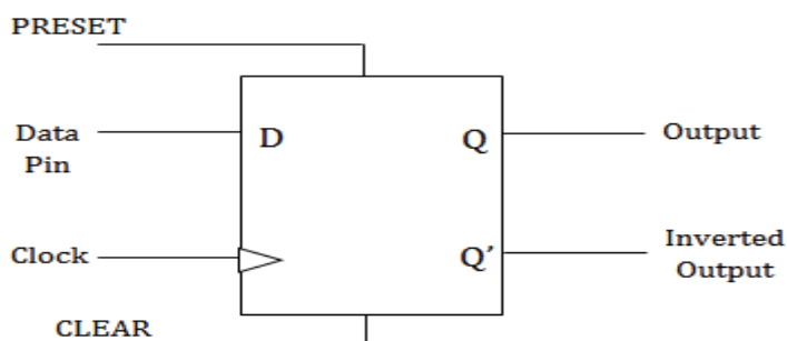
Figure 2.17 – D FF
