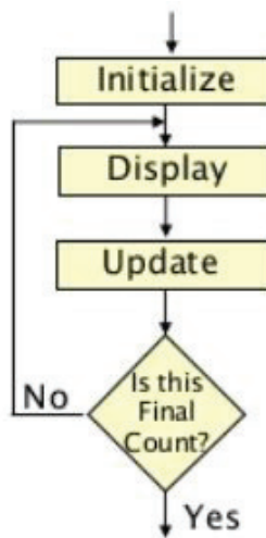
Fig. 1 Flow chart of Counter
