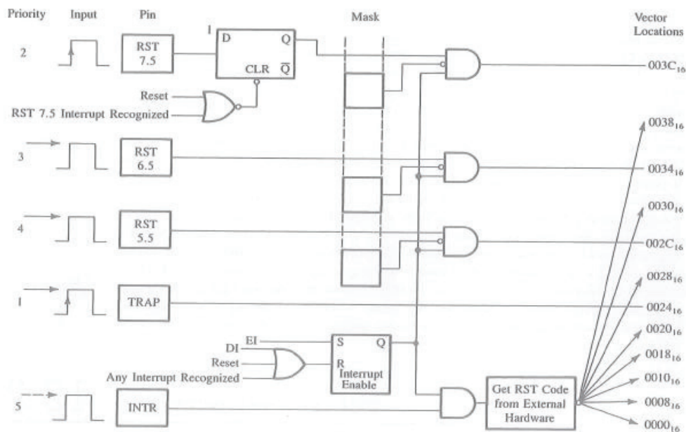
Figure 13.4 – 8085 Interrupts and Vector Location
