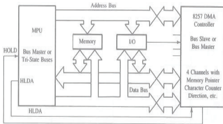
Figure 13.7 – 8257 DMA Communication
