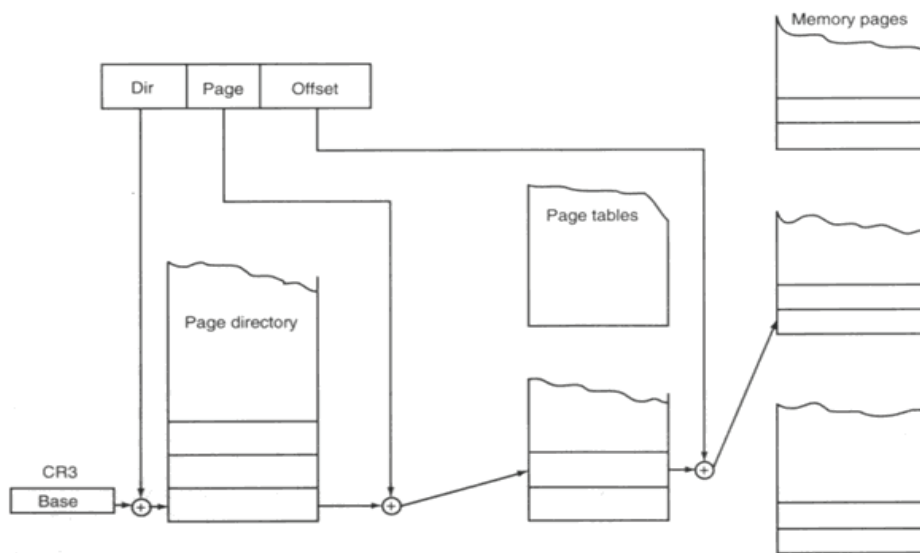
Figure 3.6: The paging mechanism the 80386, 80486, Pentium, Pentium Pro, and Pentium II microprocessor
