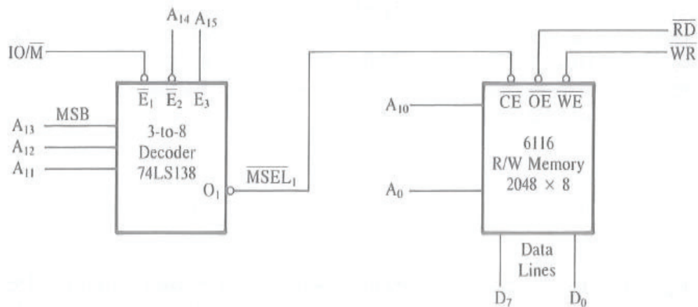
Figure 3.13 – Interfacing 2048 x 8 R/W Memory
