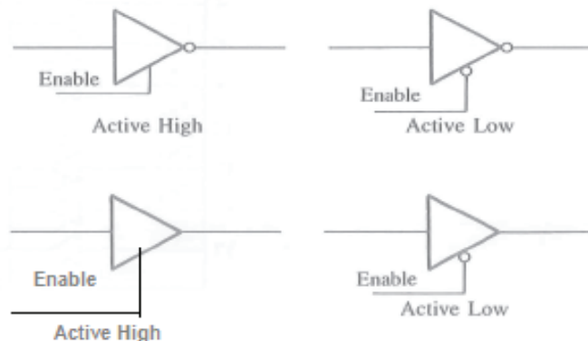
Figure 2.14 – Tristate Devices
