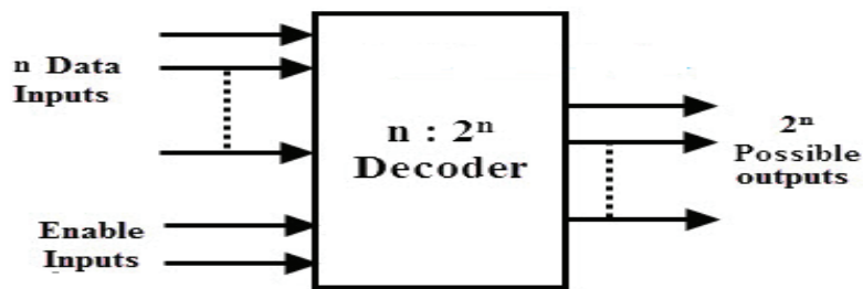
Figure 2.15 – Decoder
