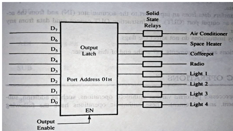
Figure 6.4: Output Port to Control Devices
