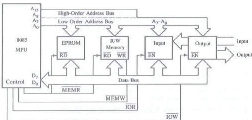
Figure 2.13 – Microcomputer System Illustration
