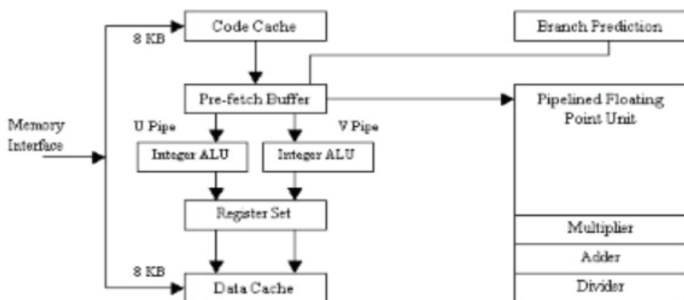
Figure 1.2: Architecture of Pentium Processor
