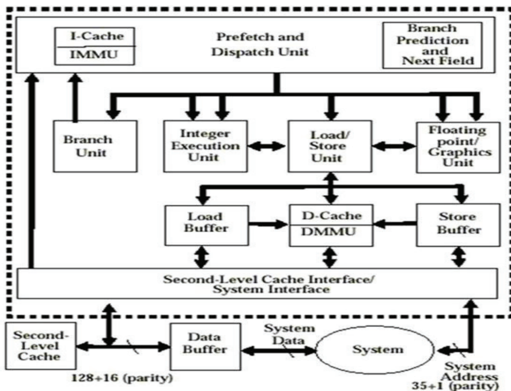
Figure 1.2: Block Diagram of Ultra SPARC
