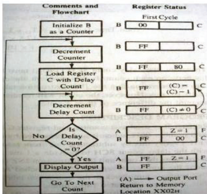
Fig 6 Flow chart for Hexadecimal Counter
