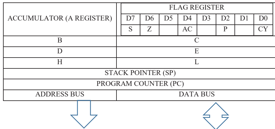
Figure 2.2 – Microprocessor internal structure
