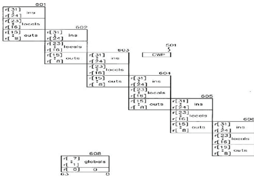
Figure 2.1: Register Window
