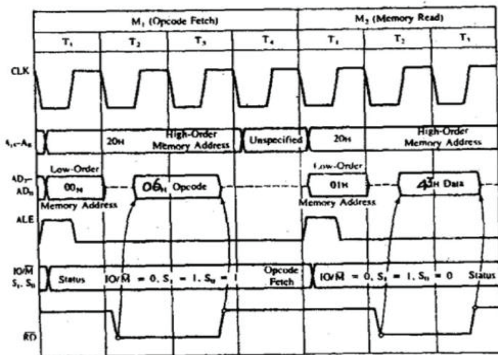
Figure 3.8 – Machine Cycles for the instruction MVI B, 43H
