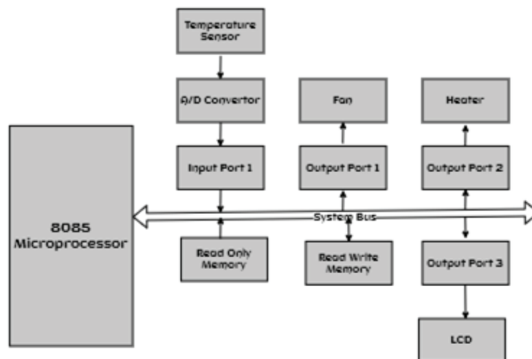
Figure 1.10 – MCTS
