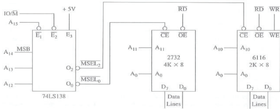
Figure 3.15 – MCTS Project Memory Interfacing
