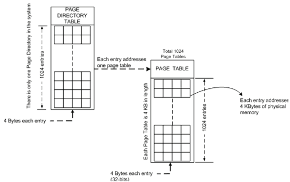
Figure 3.8: The page directory, and page table
