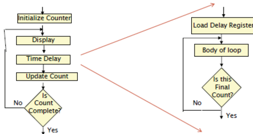
Fig 4 Counter Design with Time Delay
