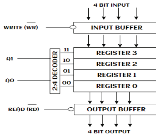
Figure 2.6 – 4 x 4 memory register block diagram
