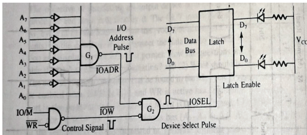
Figure 4.4:- Decoder Logic for LED Output Port
