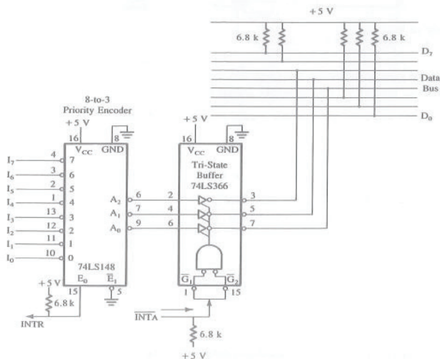
Figure 13.3 – 8:3 Priority Encoder to handle multiple interrupts
