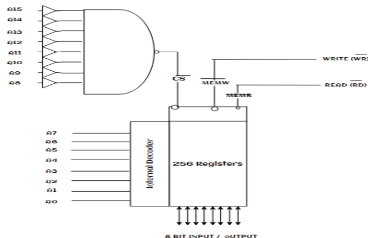
Figure 2.10 – 256 x 8 memory model
