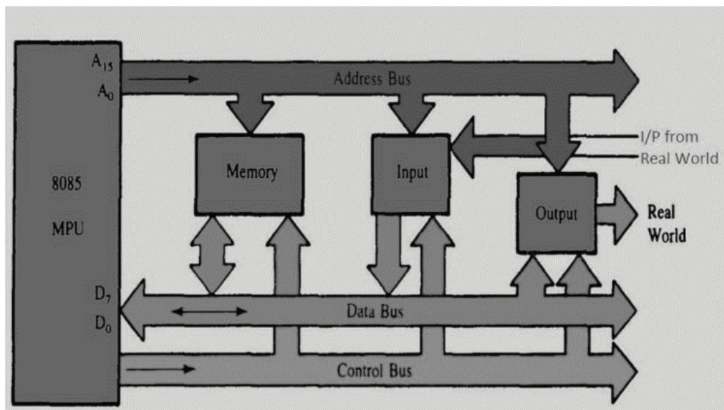
Figure 2.1 – Microprocessor and bus structure
