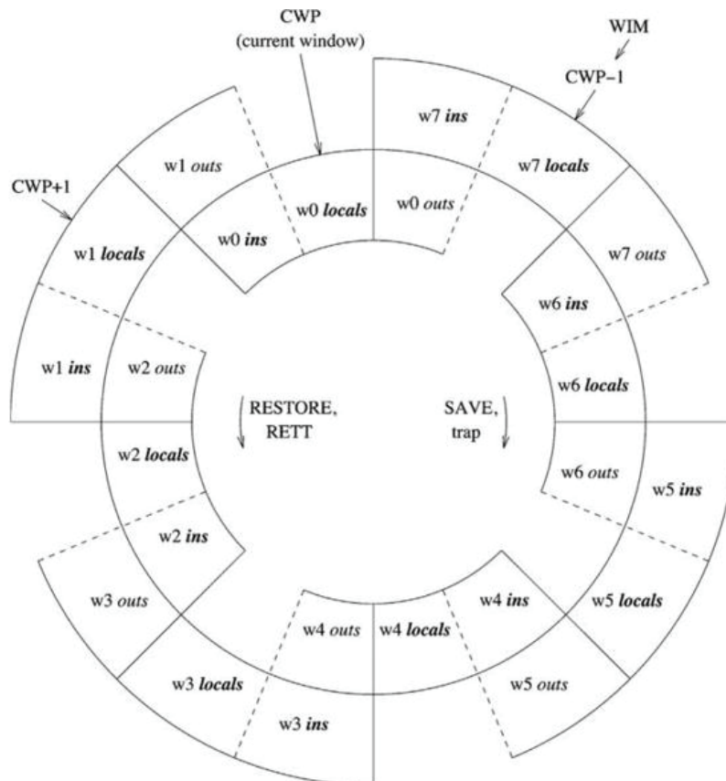
Figure 2.2: Circular Arrangement of Register Window
