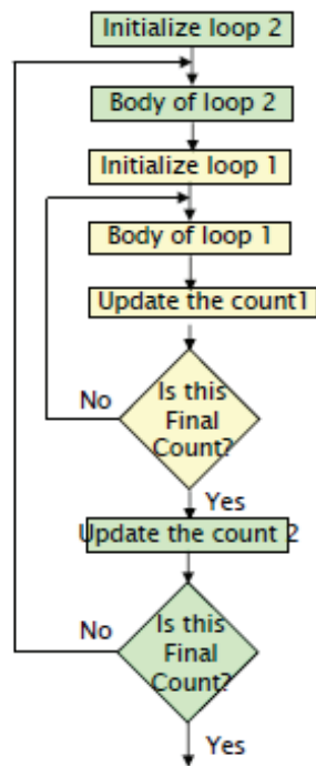
Fig 3 Flow chart for time delay with two loops
