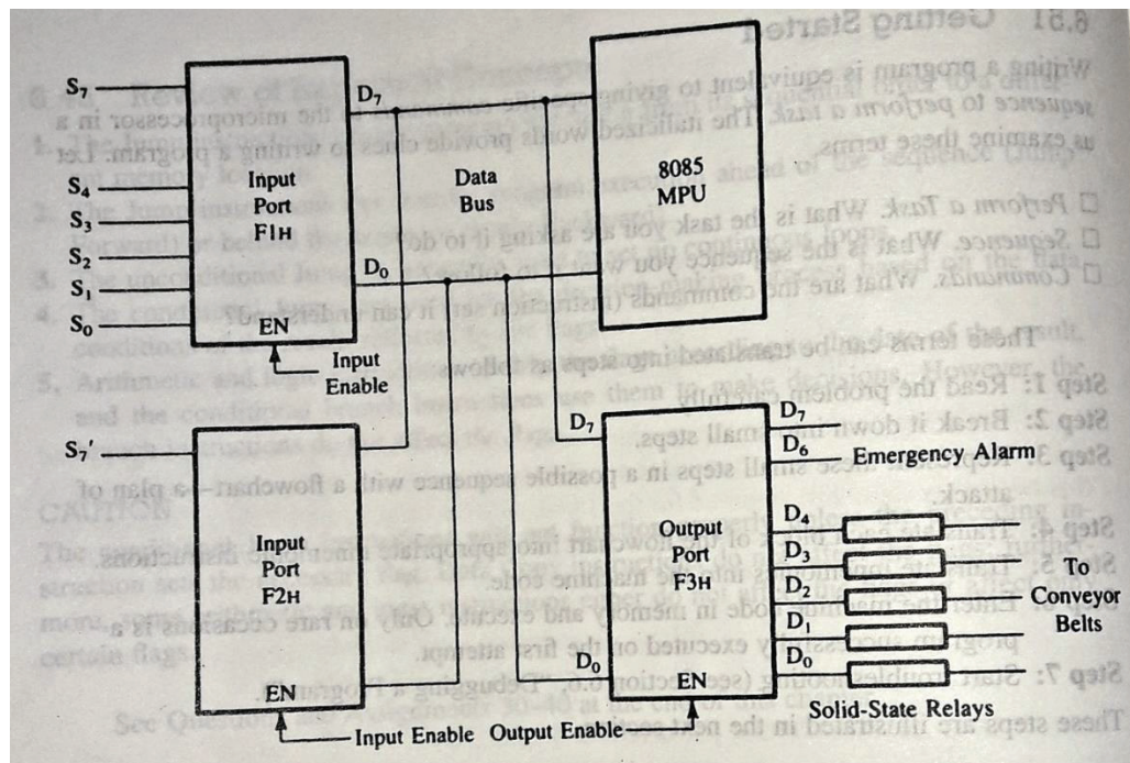
Figure 6.12: Input /Output Ports to control Manufacturing Processes
