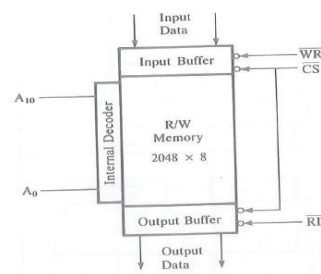
R/W Memory Chip (2048 x 8)
