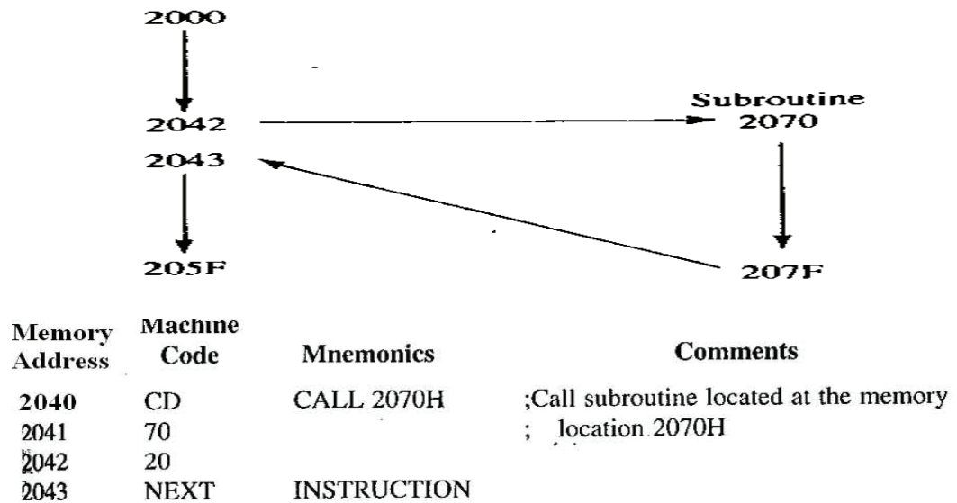
Fig. 8 - Program execution with CALL instruction
