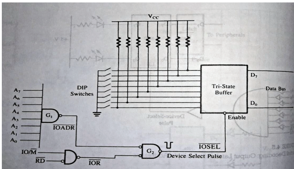
Figure 4.6 :- Decode Logic for a Dip – switch Input Port
