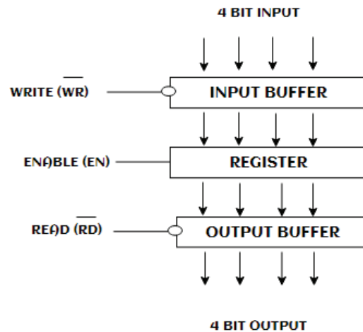
Figure 2.5 – 1 x 4 memory register block diagram
