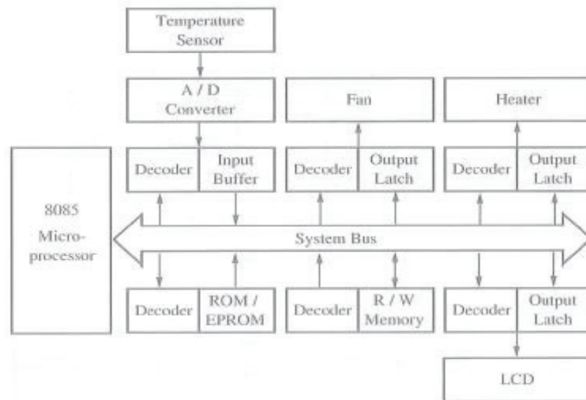
Figure 2.18 – MCTS Application
