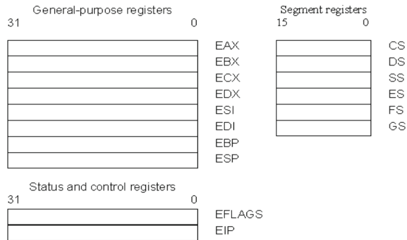
Figure 5.1: Register Set
