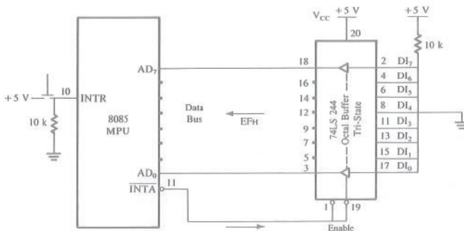
Figure 13.3 – Interrupt Implementation
