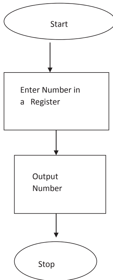
Figure 6.2 : Flowchart
