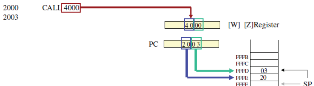
Fig 5 CALL Instruction
