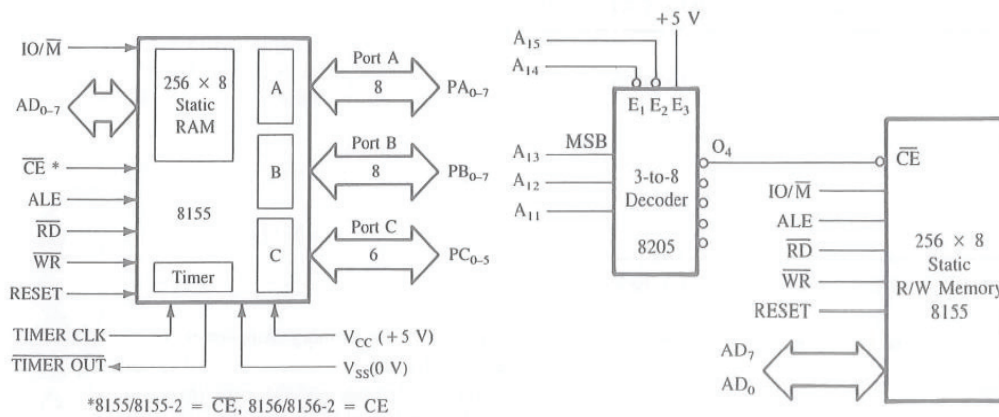
Figure 3.14 – 8155 Memory and SDK-85
