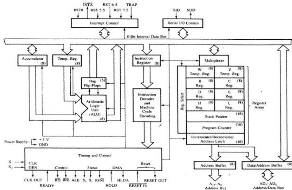
Figure 3.5 – 8085 Architectural Block Diagram
