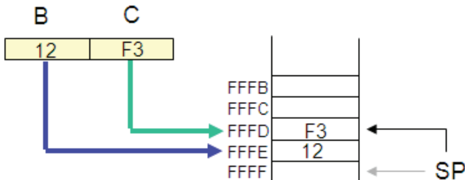
Fig 2. Push Operation of Stack
