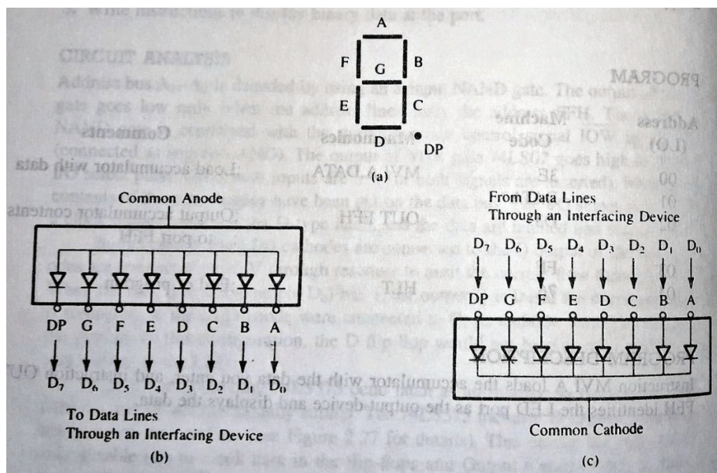
Figure 4.9 :- Seven-Segment LED : LED Segments(a) ;Common-Anode LED(b); Common- Cathode LED (c)
