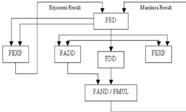
Figure 1.4: Floating Point Unit
