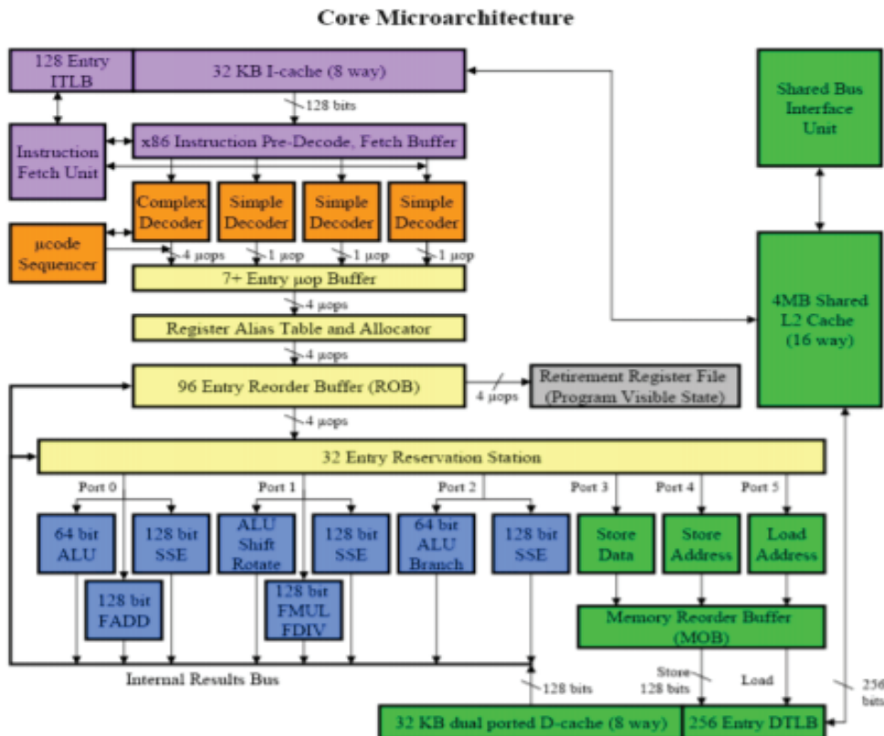
Figure 4.1: Intel Core Microarchitecture
