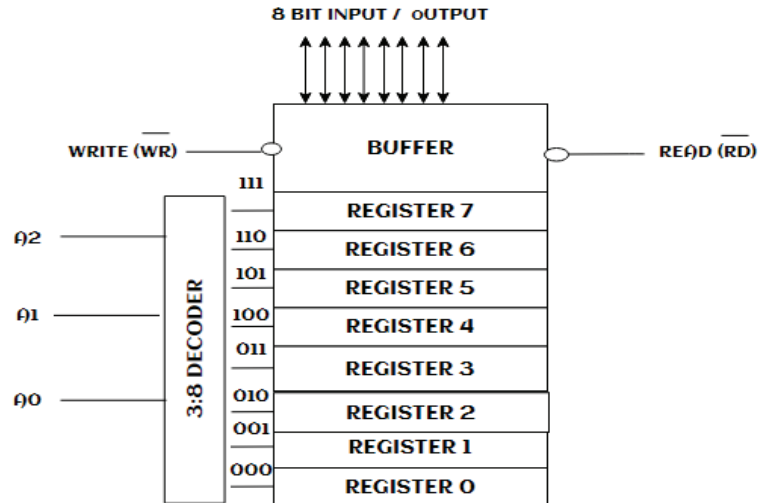
Figure 2.7 – 8 x 8 memory register block diagram
