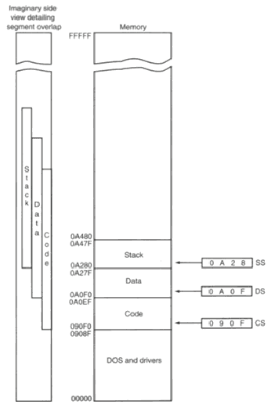
Figure 3.3: An Application program containing code, data and stack segment loaded into DOS system memory
