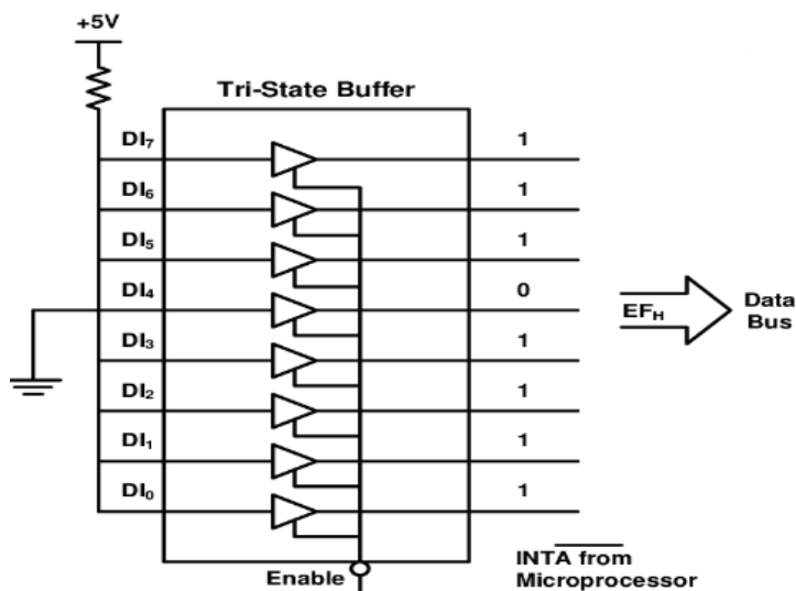
Figure 13.1 – RST 5 Circuit
