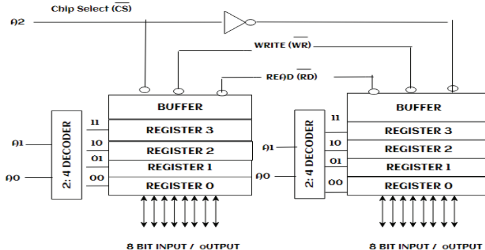
Figure 2.8 – 8 x 8 memory register with chip select
