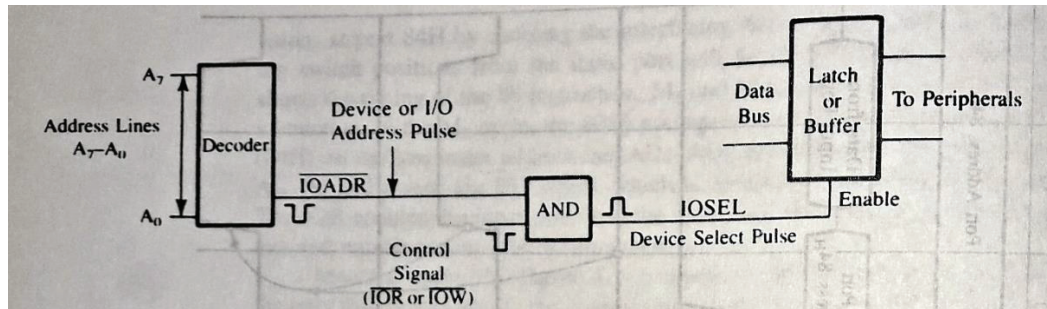
Figure 4.3 :- Block Diagram of I/O Interface
