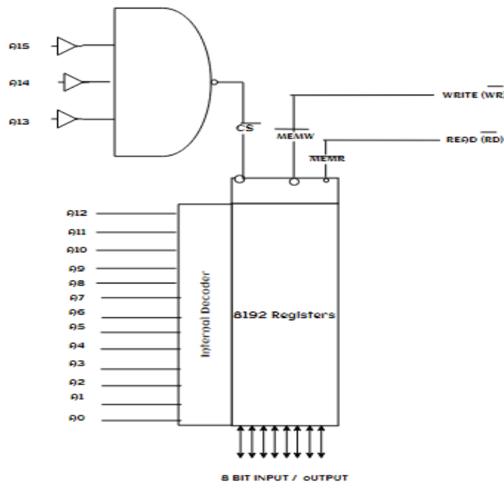
Figure 2.11 – 8192 x 8 memory model
