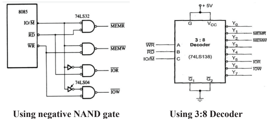
Figure 3.4 – Generating the control signal
