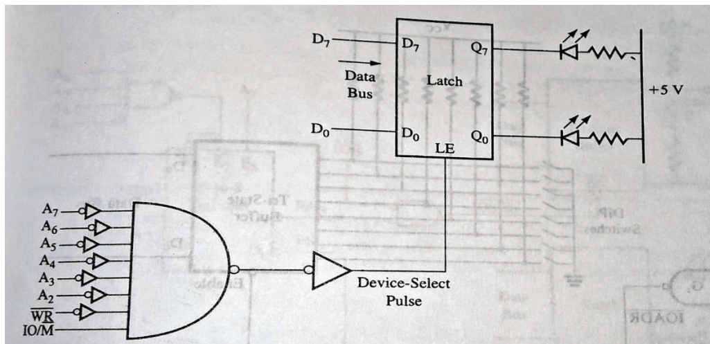
Figure 4.5 :- Partial Decoding : Output Latch with Multiple Addresses
